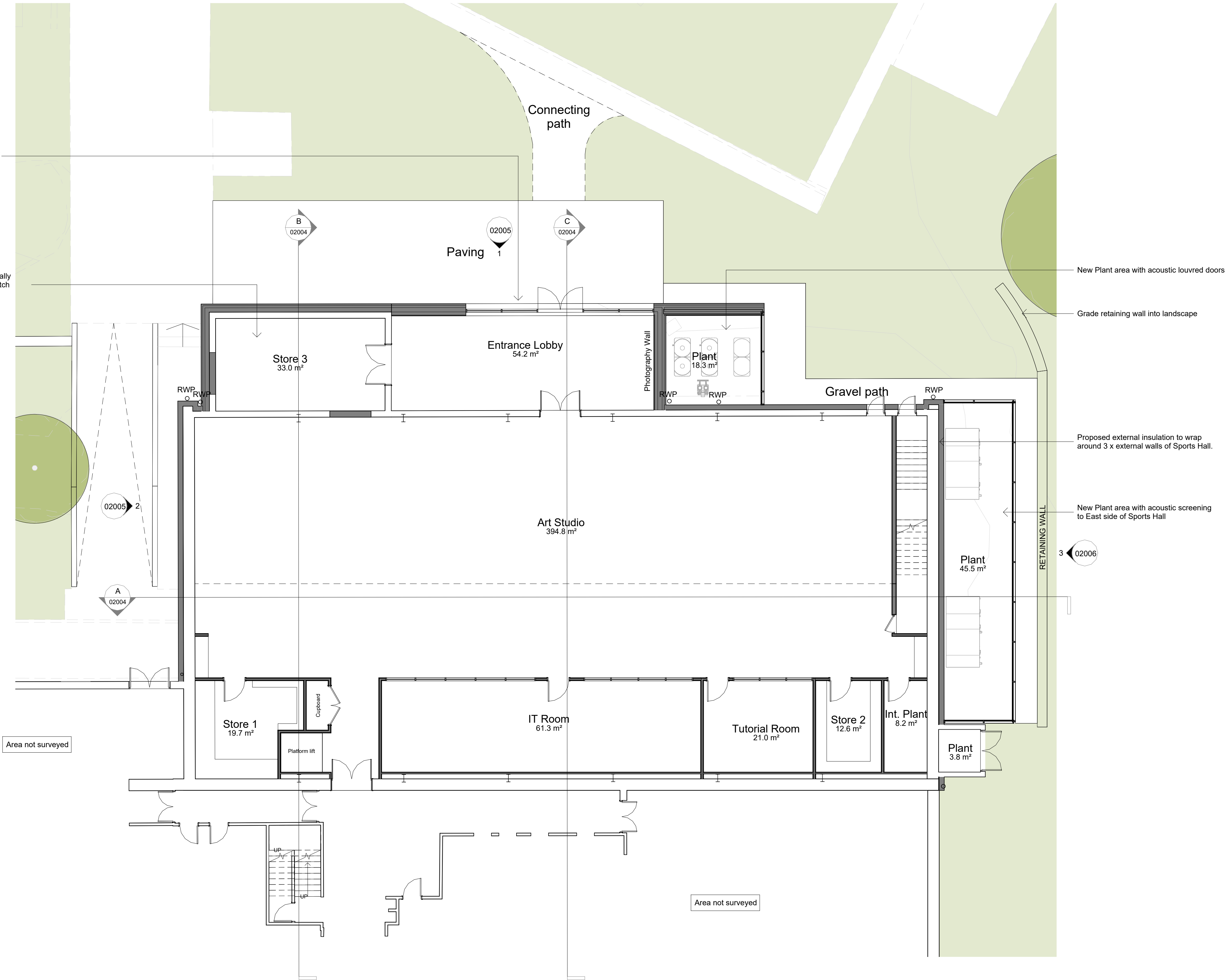
Proposed Sports Hall - Ground Floor Plan 1 : 100
