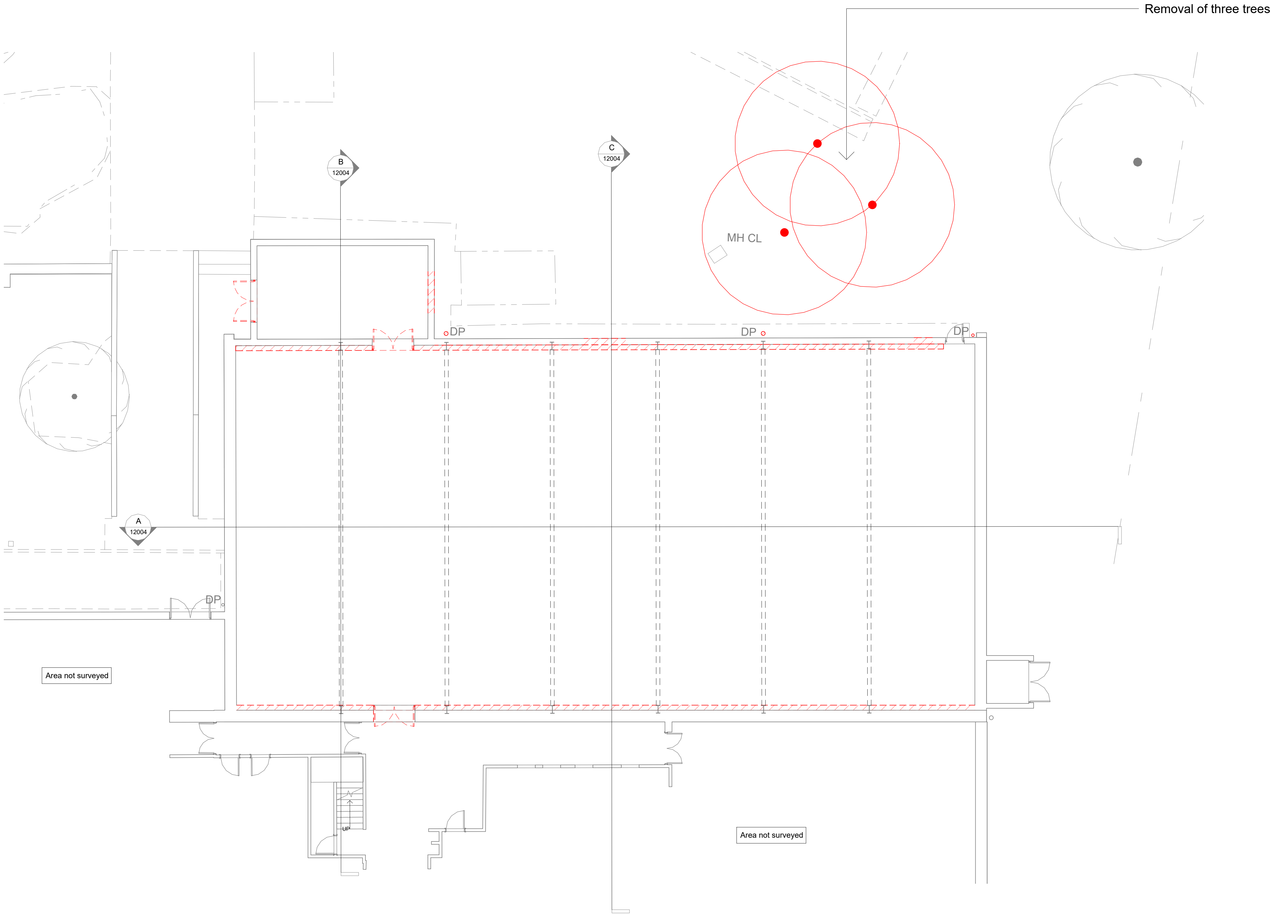
Demolition Sports Hall - Ground Floor Plan 1 : 100
