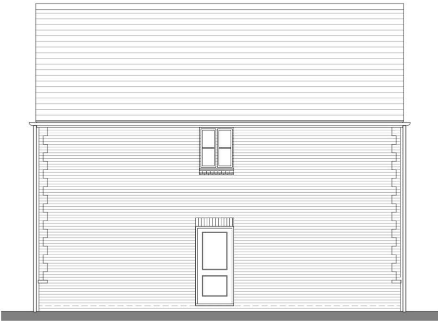
Rear Elevation
