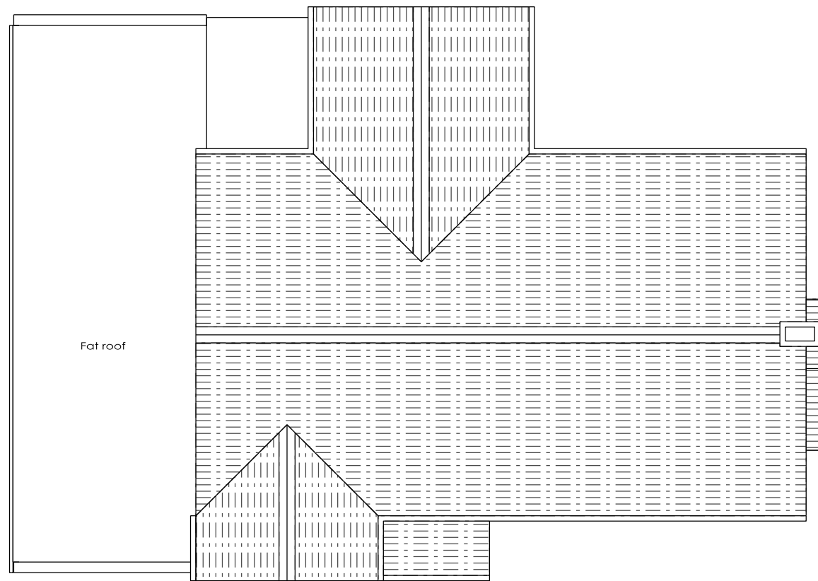
ROOF PLAN 1:100
