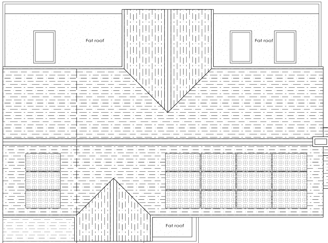
ROOF PLAN 1:100
