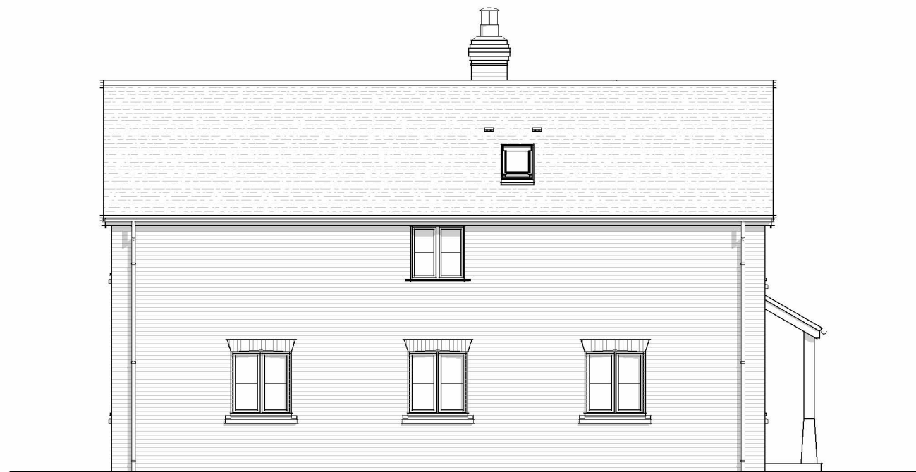
Side 1 Elevation (Planning) 1 : 100
