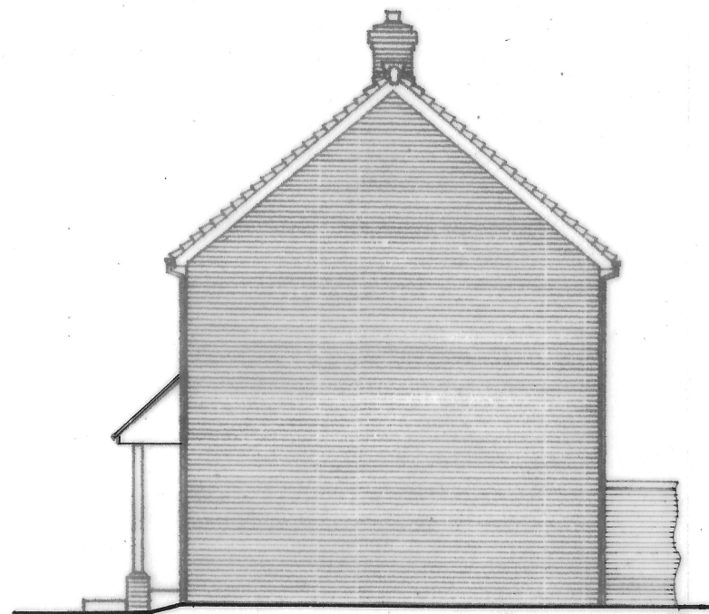
PROPOSED NORTH ELEVATION
