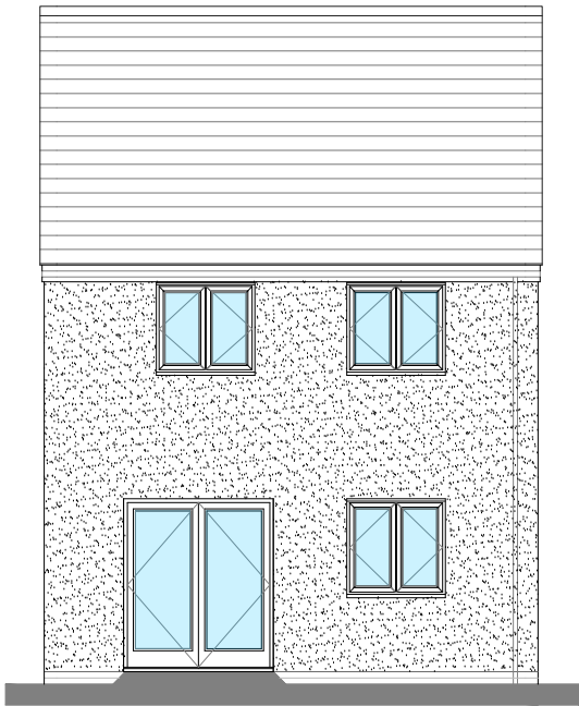
REAR ELEVATION
