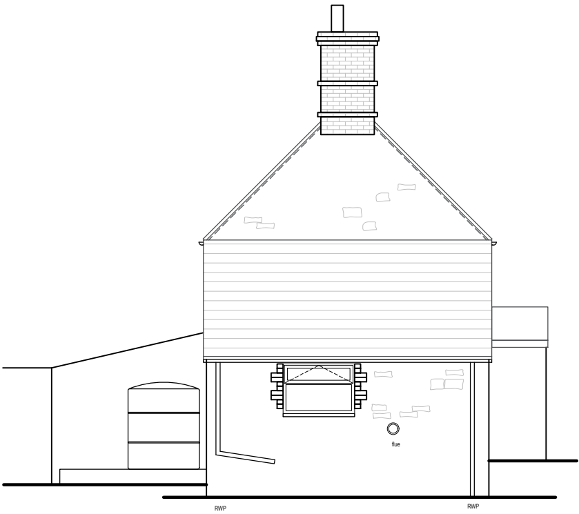
EXISTING NORTH WEST ELEVATION
