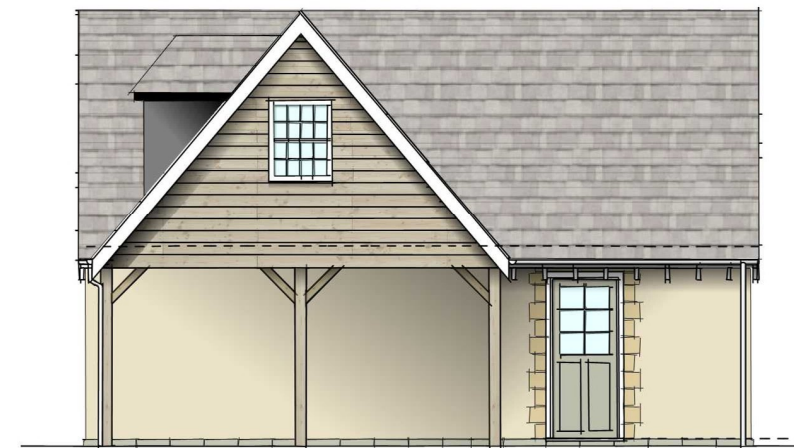
EAST ELEVATION
