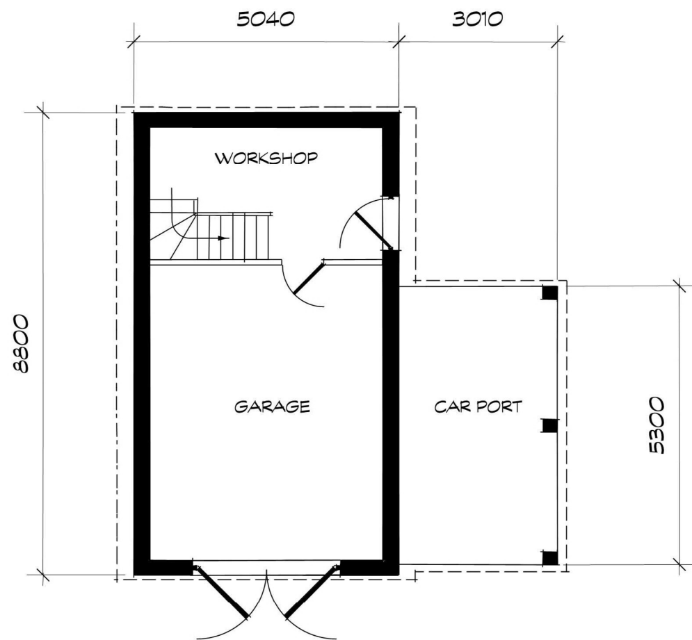
PLAN - GROUND FLOOR
