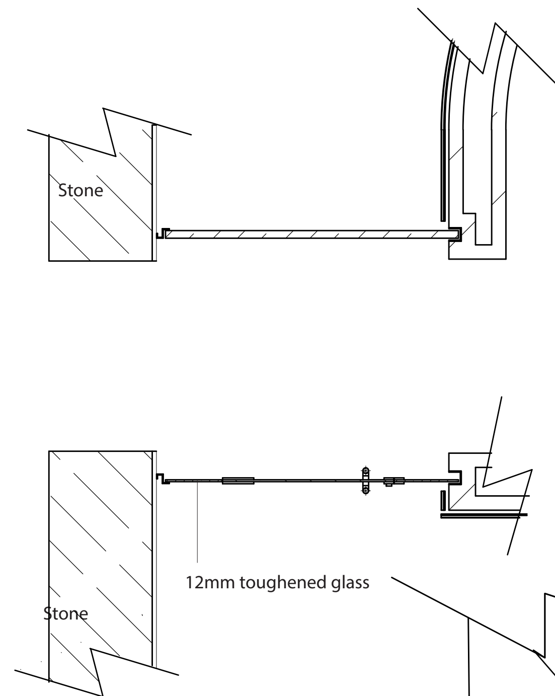
Section B-B at Ground floor Level Scale 1:10
