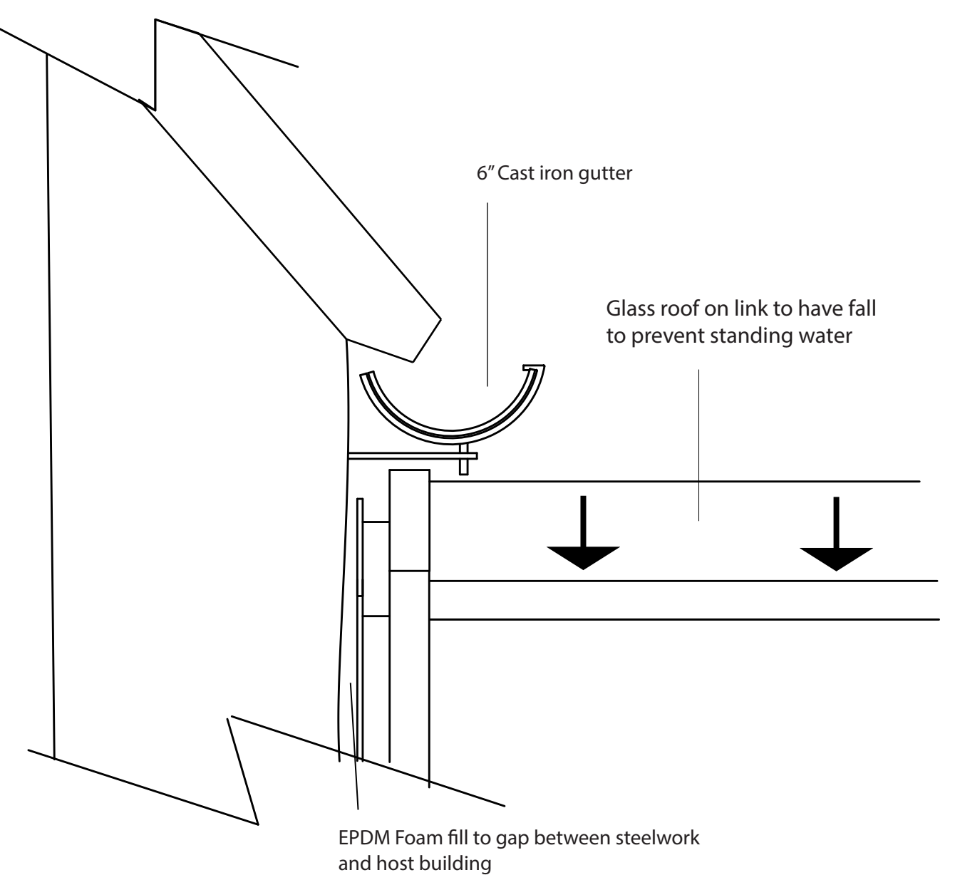
Detail view showing junction between stone wall and glass link Scale 1:5
