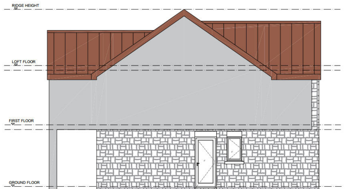
SIDE ELEVATION 2 AS PROPOSED
