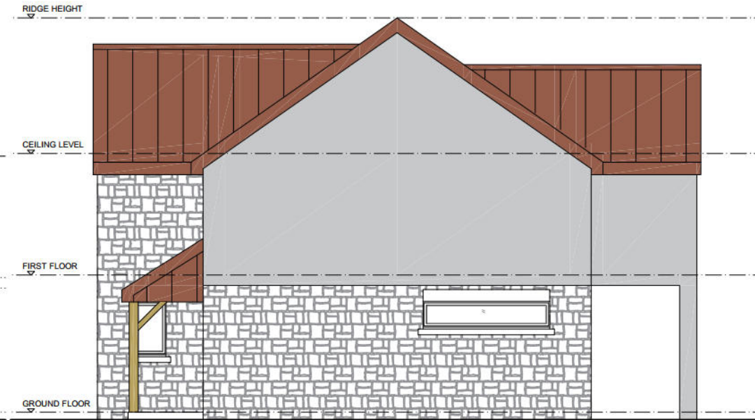
SIDE ELEVATION 1 AS PROPOSED
