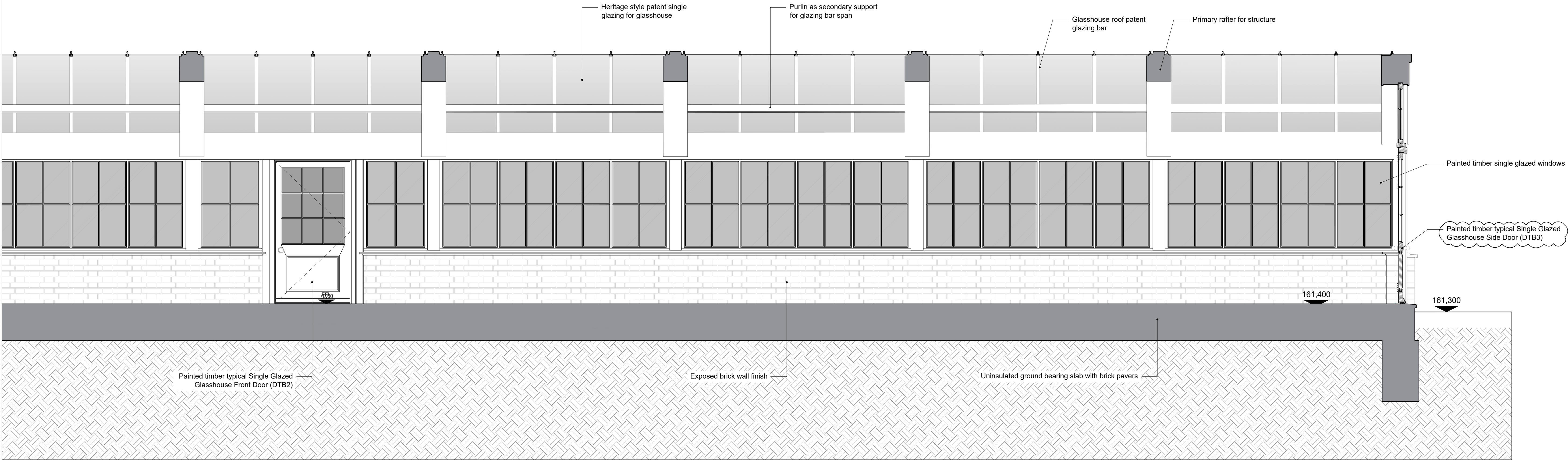
266 Buildings 18 & 19 - Proposed Section B-B 1:25_@_A1
