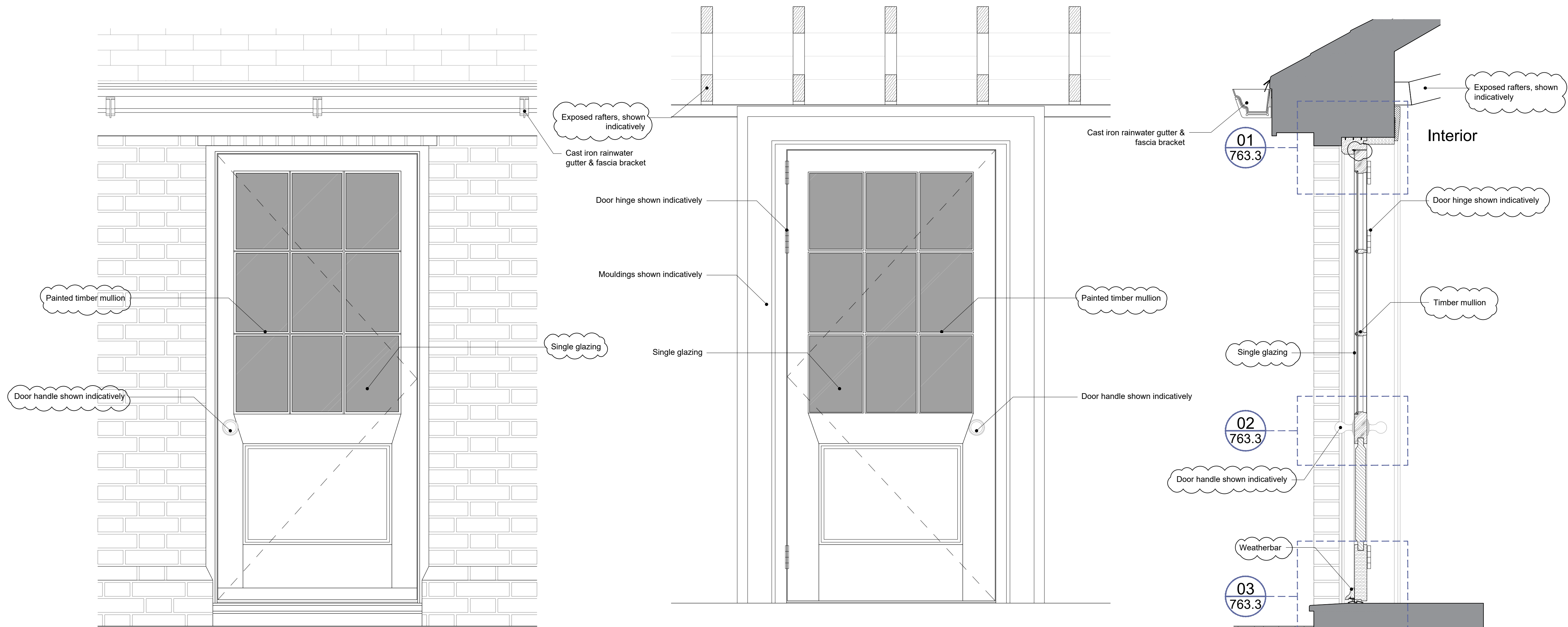
02 Door Type B9 - Typical Panelled Timber and Single Glazed Door External Elevation 763.1 SCALE 1:10 @ A1
