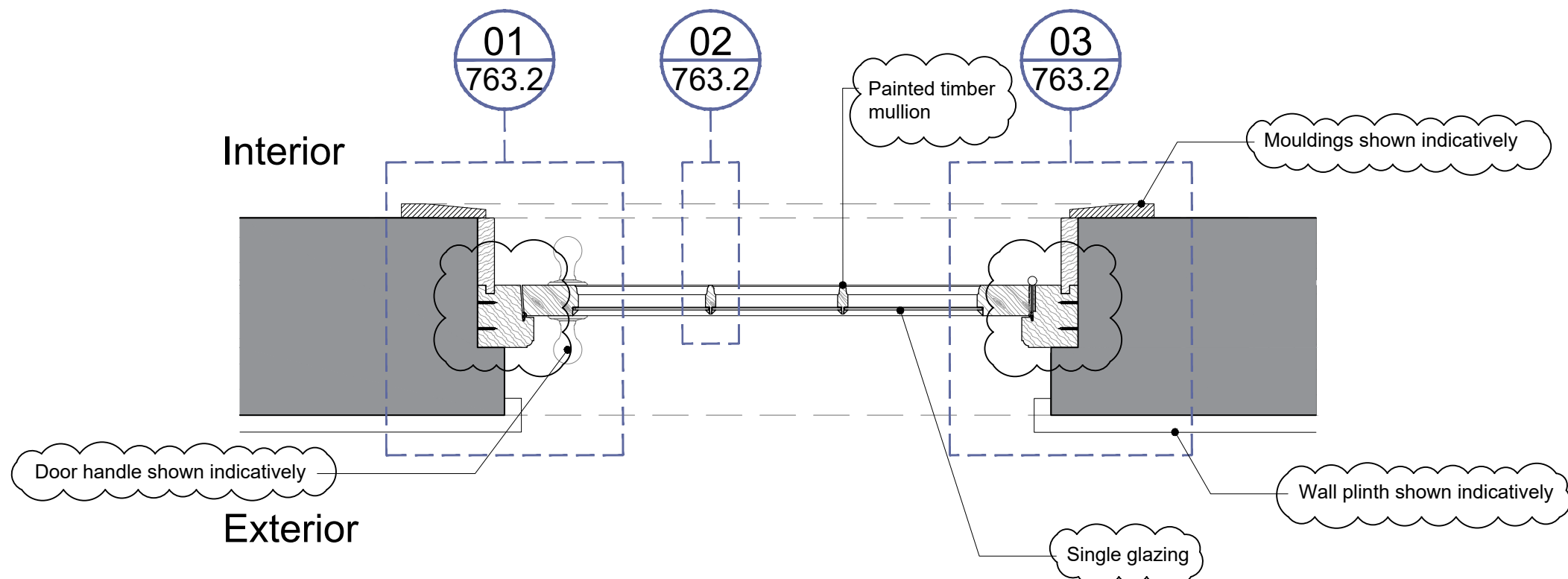
01 Door Type B9 - Typical Panelled Timber and Single Glazed Door Plan 763.1 SCALE 1:10 @ A1
