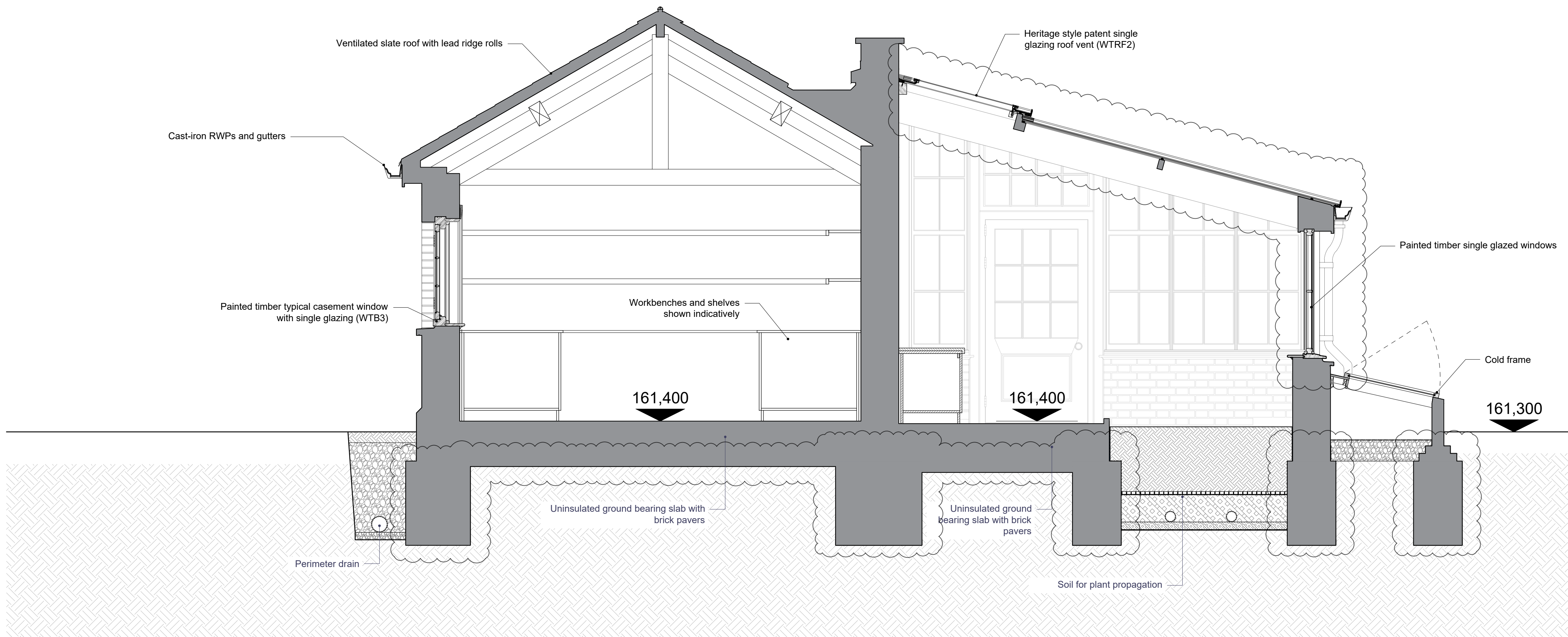
265 Buildings 18 & 19 - Proposed Section A-A 1:25_@_A1
