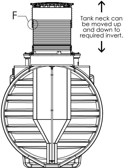
SECTION E-E SCALE 1 : 25
