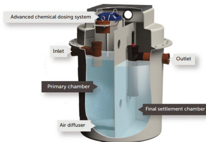
Figure 10 Aqua-Purative-G-APS 3D cutaway showing two chambers
