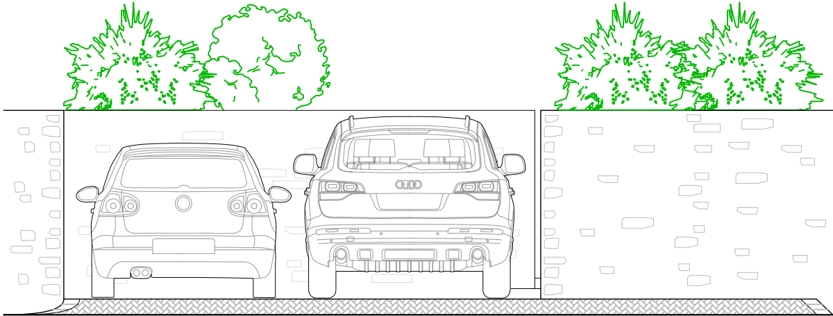
PROPOSED STREET ELEVATION
