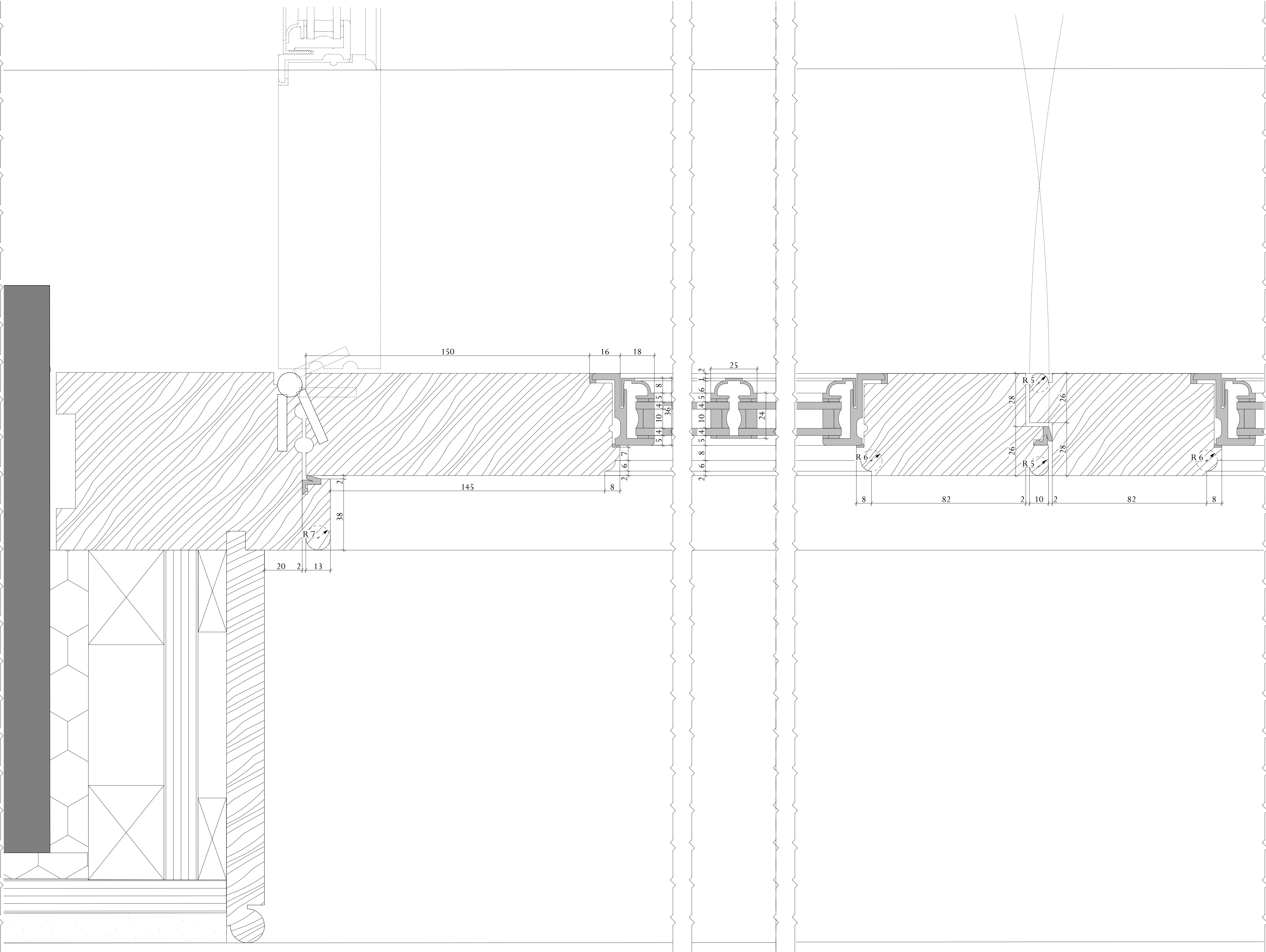
FULL SCALE DOOR REVEAL DETAIL PLAN 1 SCALE 1:1
