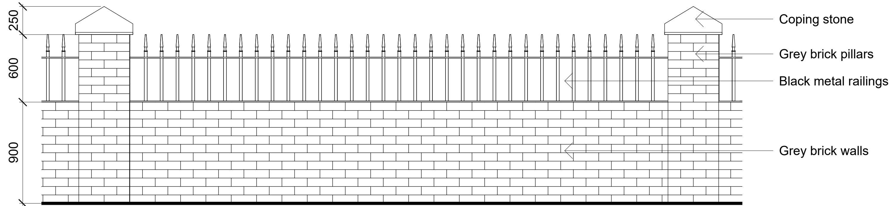
Elevation of Boundary Wall 1 : 20
