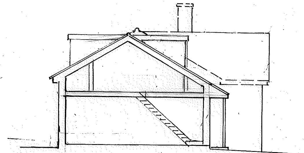
SECTION THRO' EXTENSION 1:100
