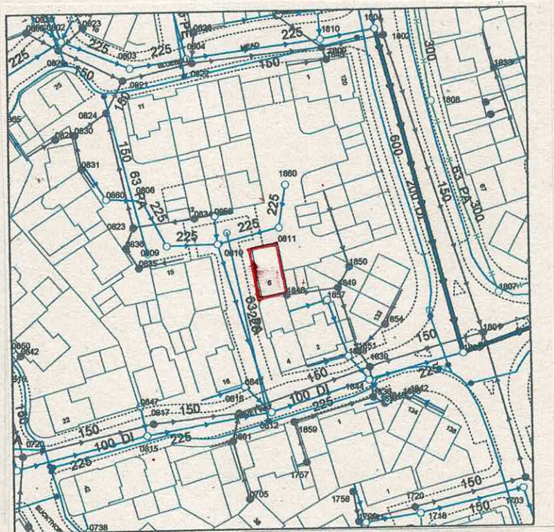
Location Plan 1:1250
