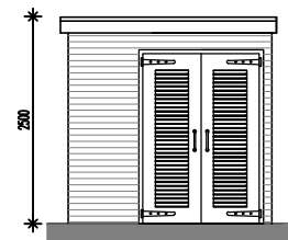
Front Elevation
