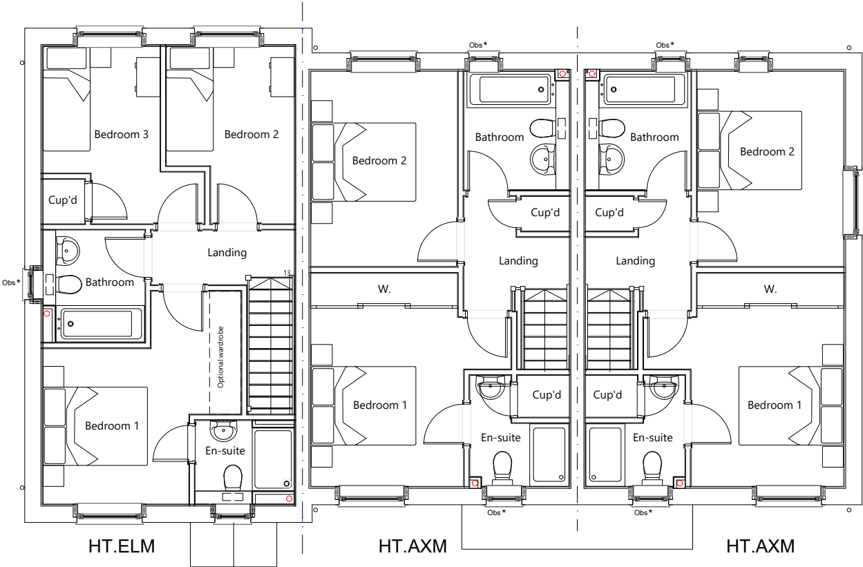
First Floor Plan Obs* - Obscure Window
