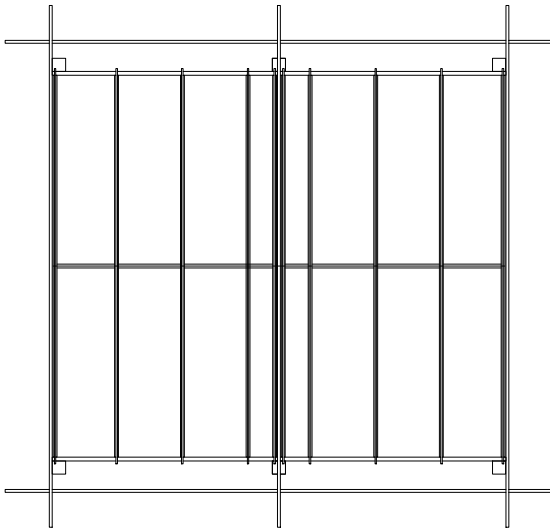
Roof Plan
