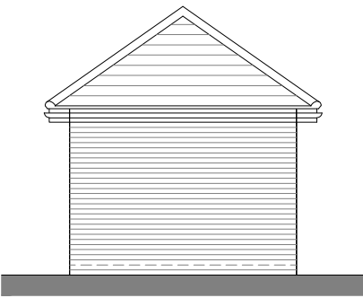
Rear Elevation
