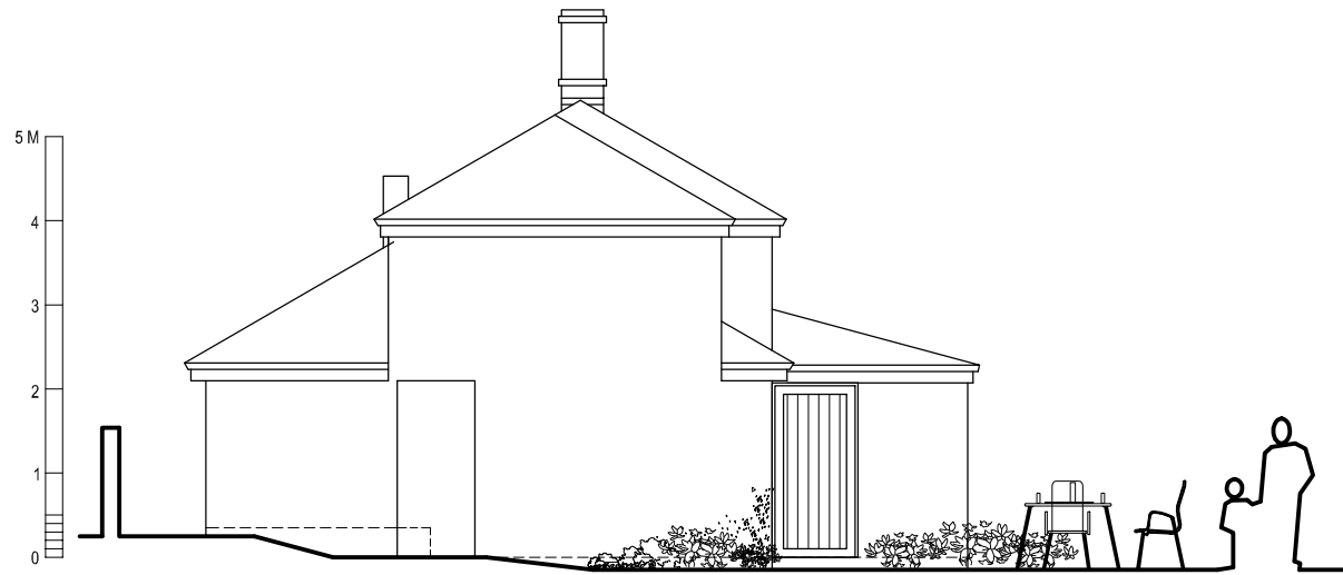
PROPOSED SIDE NORTH-WEST ELEVATION
