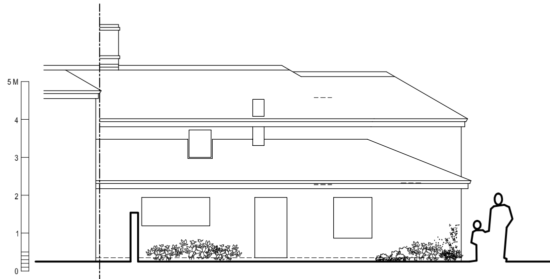
PROPOSED REAR NORTH-EAST ELEVATION
