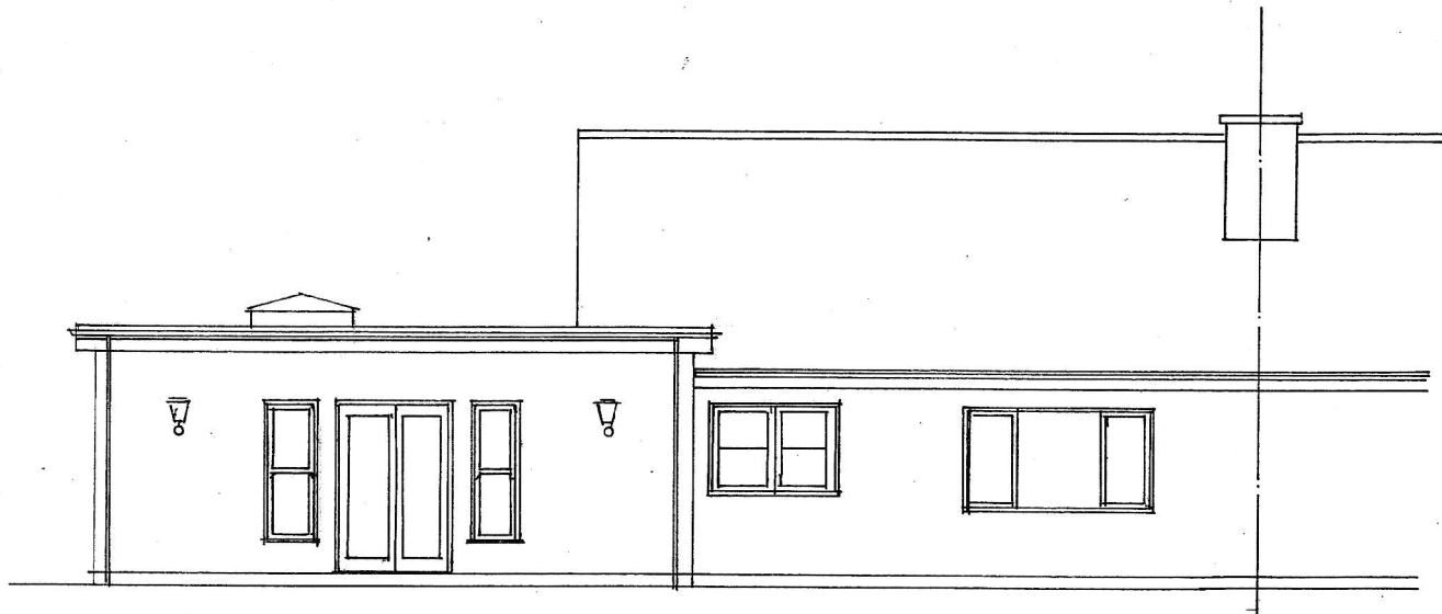
REAR
