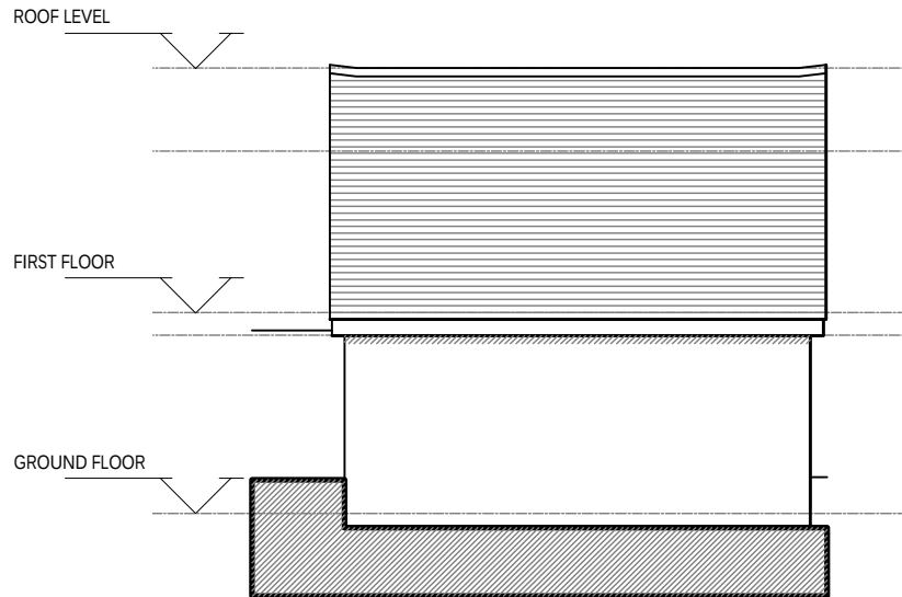
EXISTING SOUTH ELEVATION 1:100 @ A4
