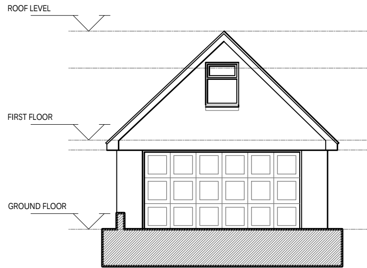
EXISTING EAST ELEVATION 1:100 @ A4
