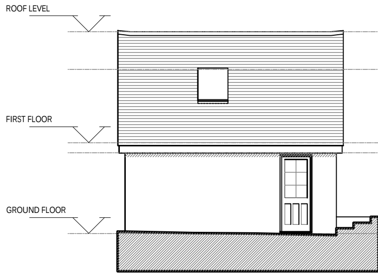
EXISTING NORTH ELEVATION 1:100 @ A4
