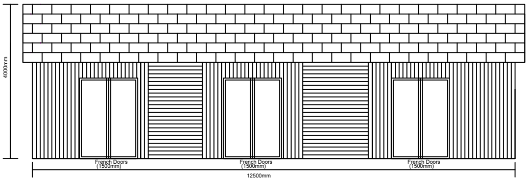
Southeast Elevation
