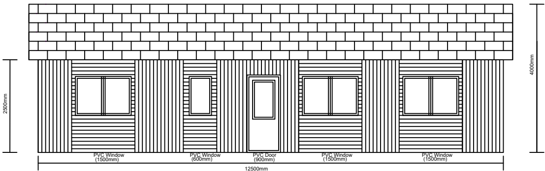
Northwest Elevation
