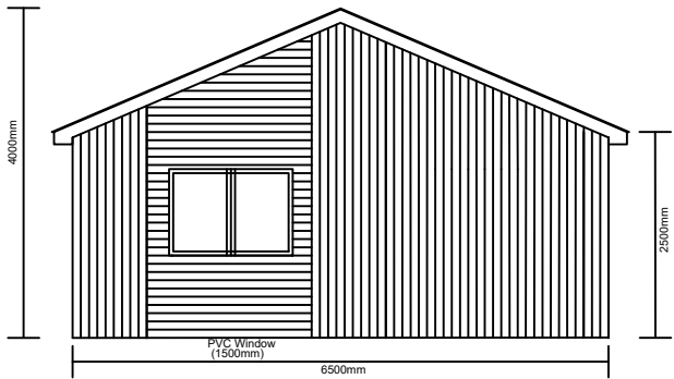
Northeast Elevation
