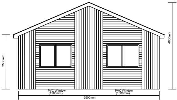
Southwest Elevation
