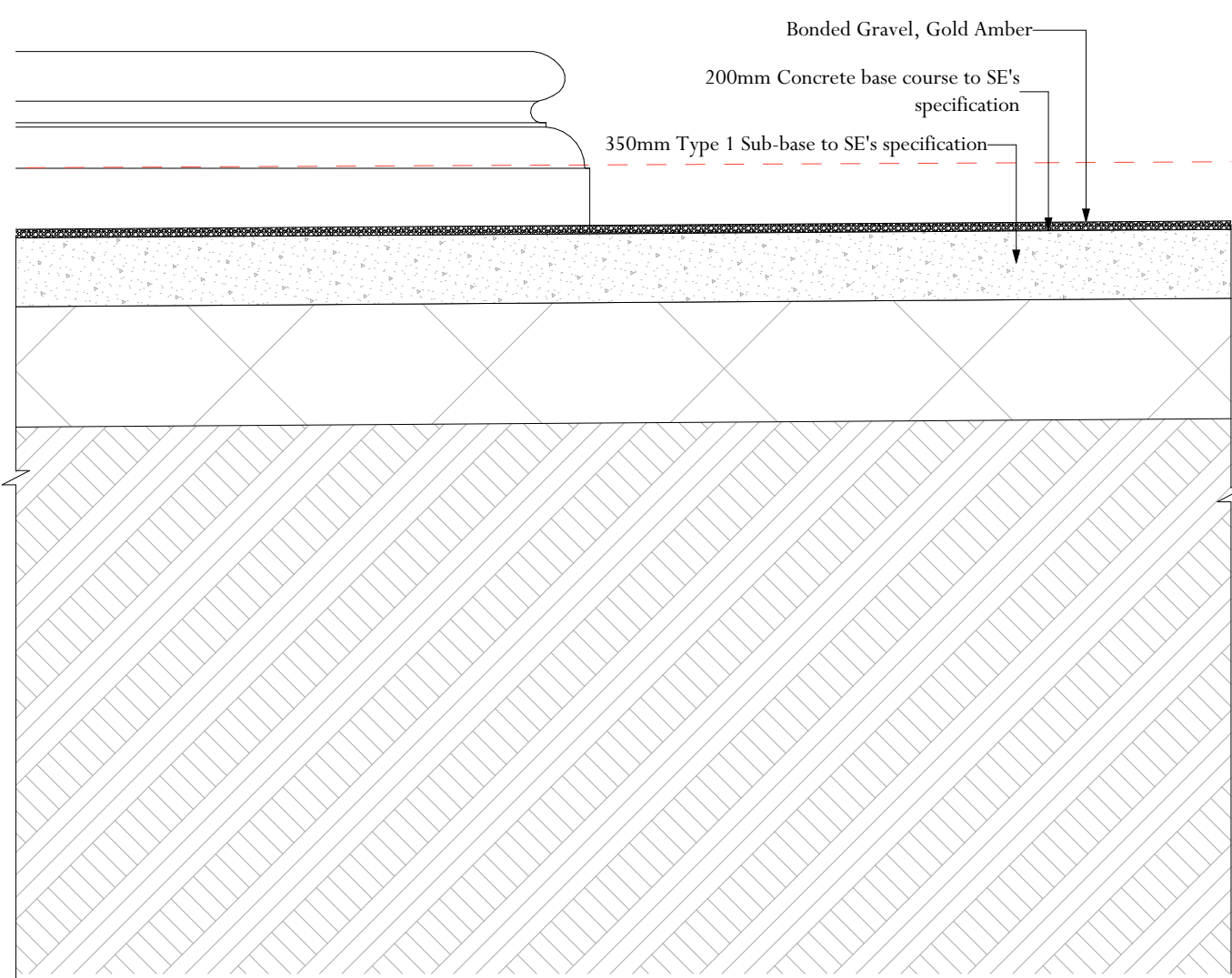
C-C Forecourt, Detail 1
