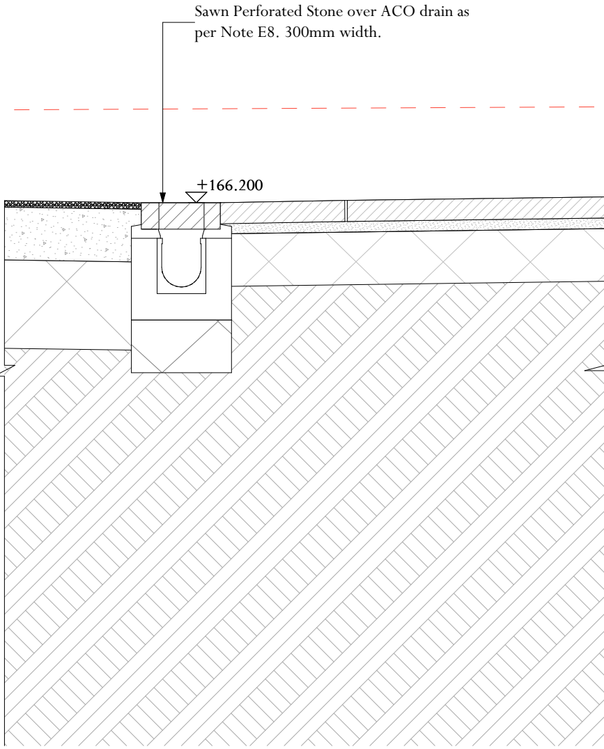
C-C Forecourt, Detail 2
