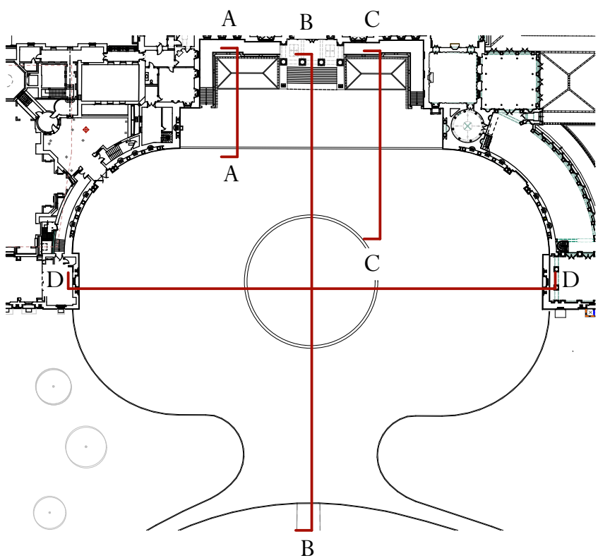
Forecourt Key Plan
