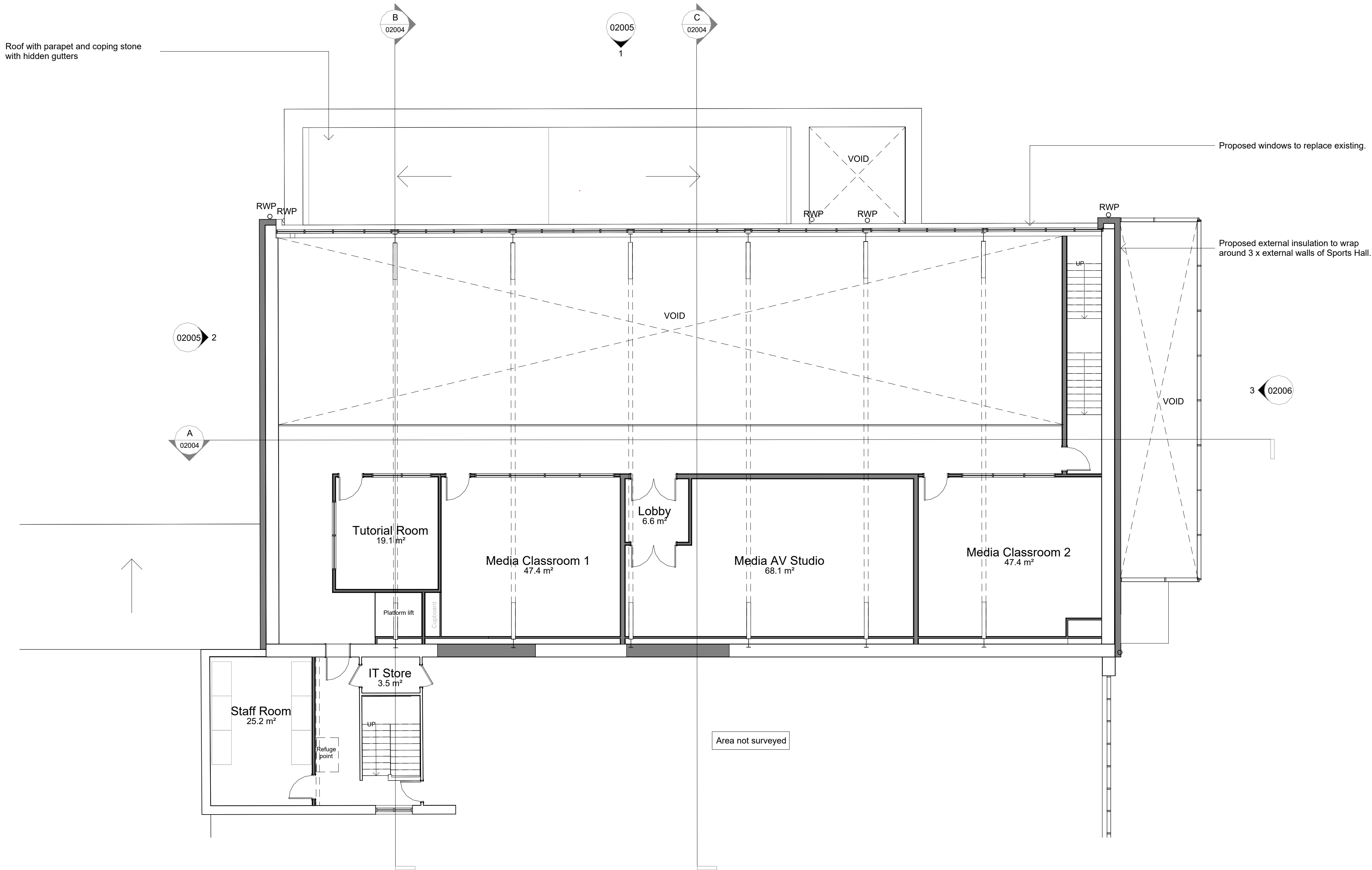
Proposed Sports Hall - First Floor Plan 1 : 100
