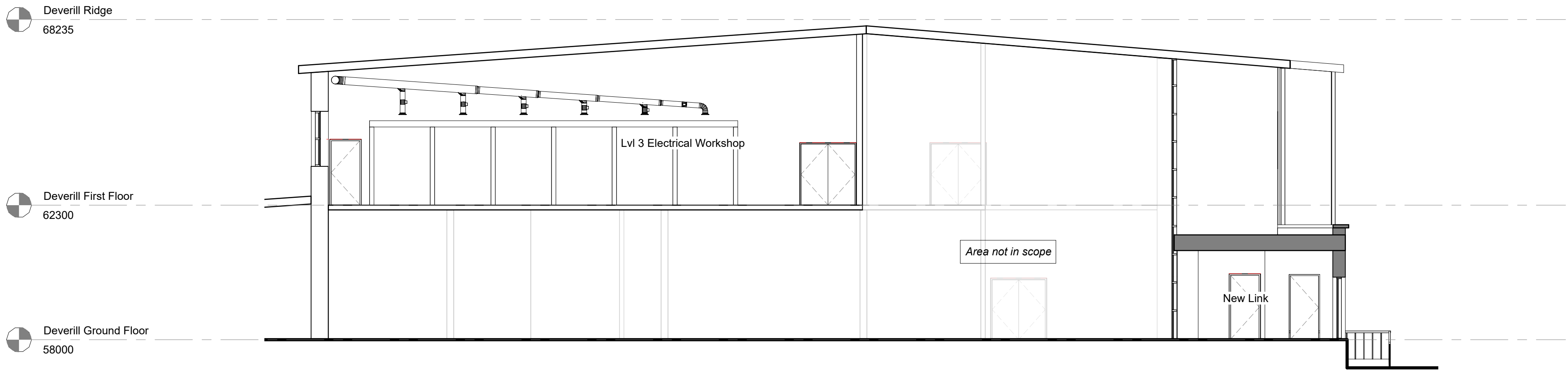
Proposed Deverill Building - Section C 1 : 100
