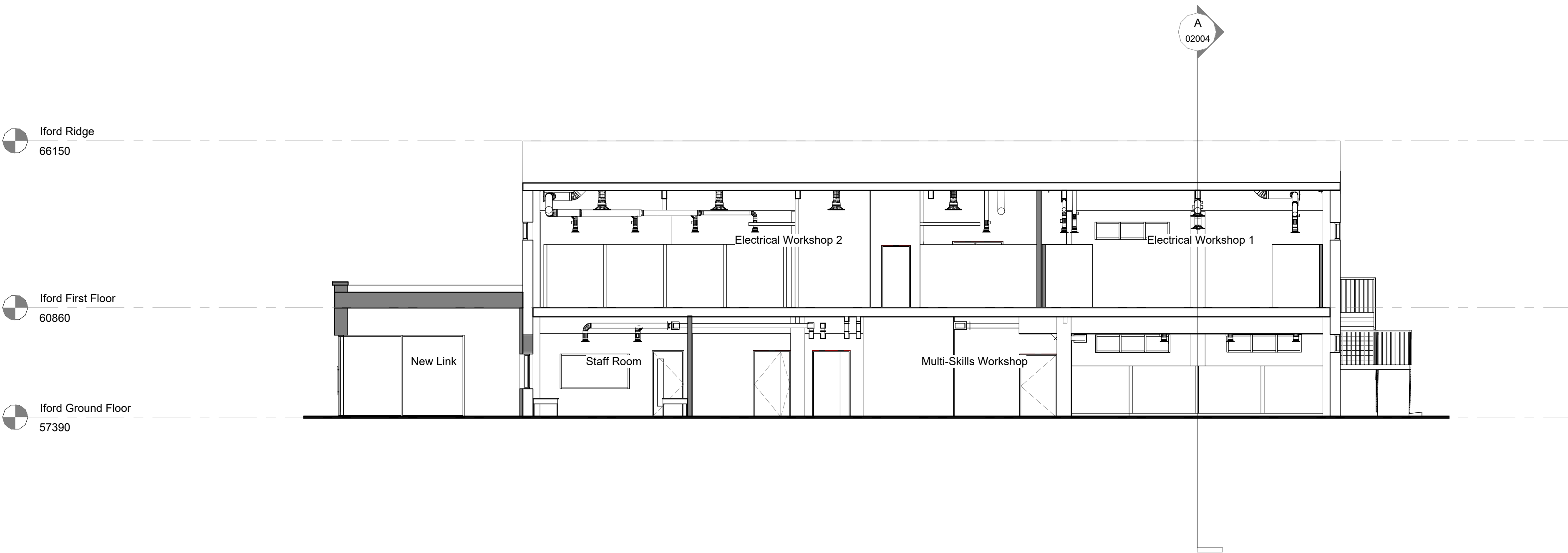
Proposed Iford Building - Section B 1 : 100
