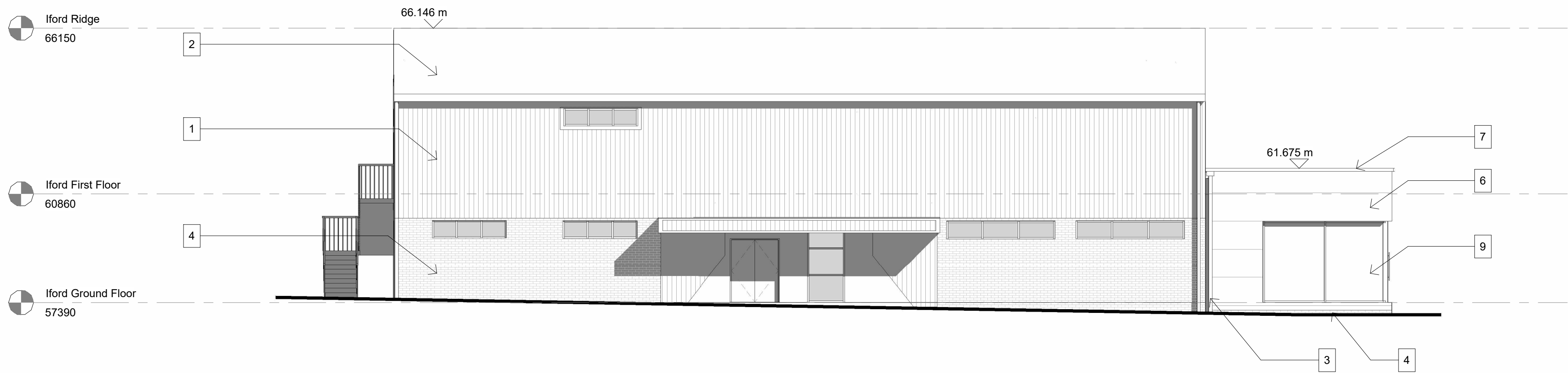
Proposed Iford Building - Elevation 2 (Front) & Side Elevation of New Link 1 : 100
