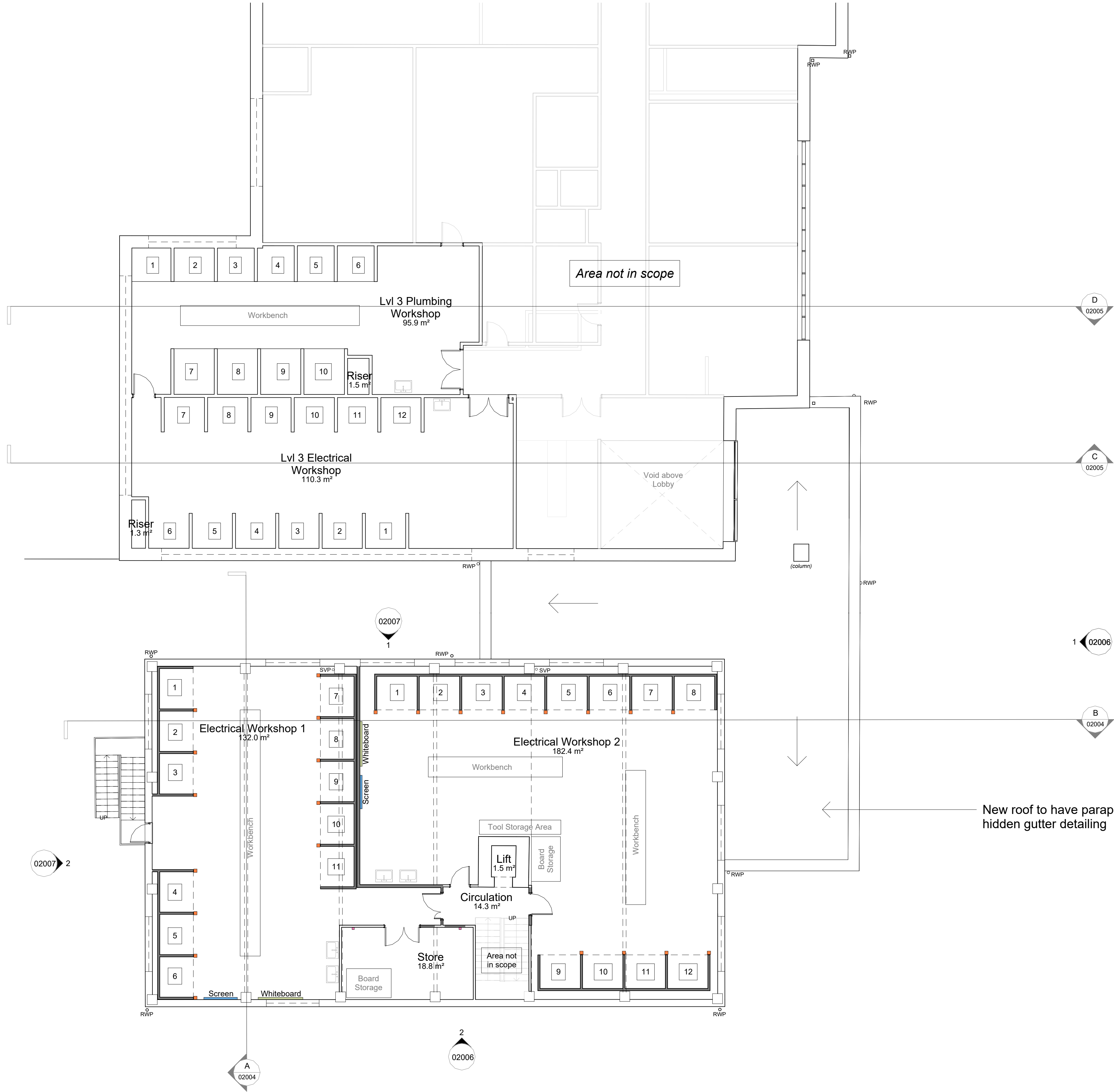
Proposed Iford & Deverill - First Floor Plan 1 : 100
