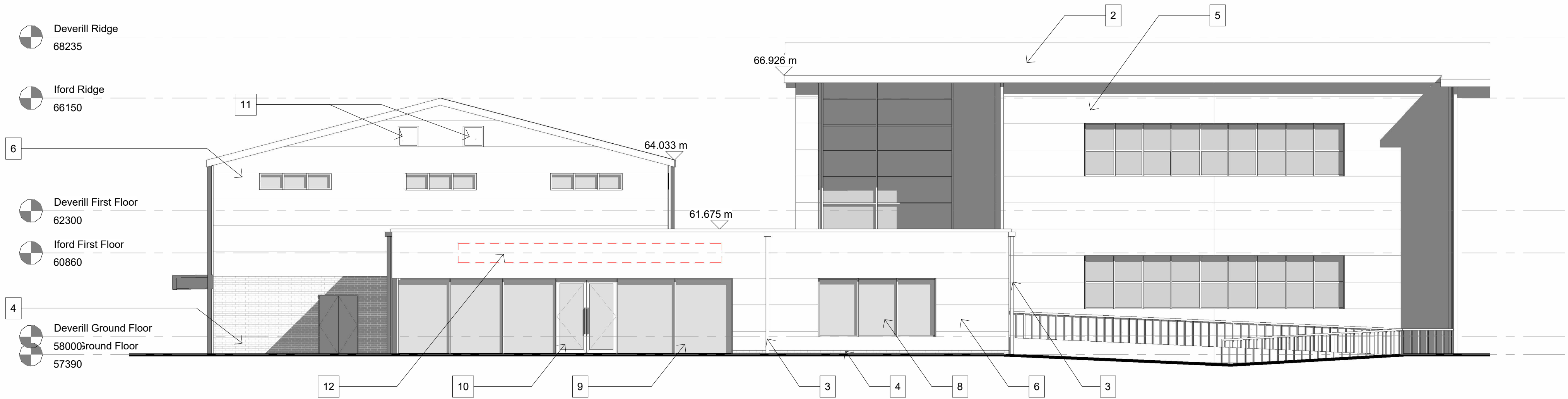
Proposed Iford & Deverill - Elevation 1 1 : 100
