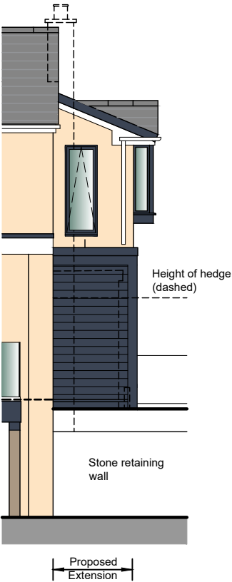
Part South West Elevation
