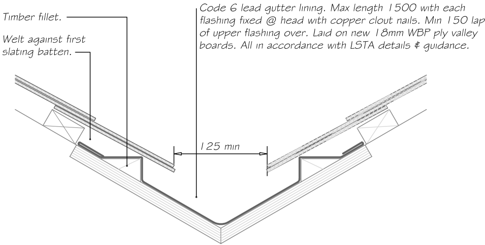
TYPICAL PITCHED VALLEY GUTTER DETAIL
