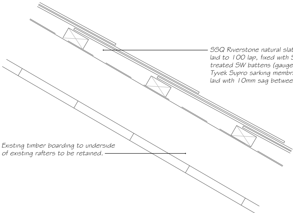
TYPICAL ROOF DETAIL
