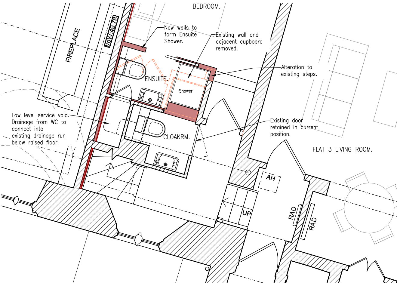
FLAT 3 FIRST FLOOR, WC/ENSUITE ALTERATION, SCALE 1:50@A2.
