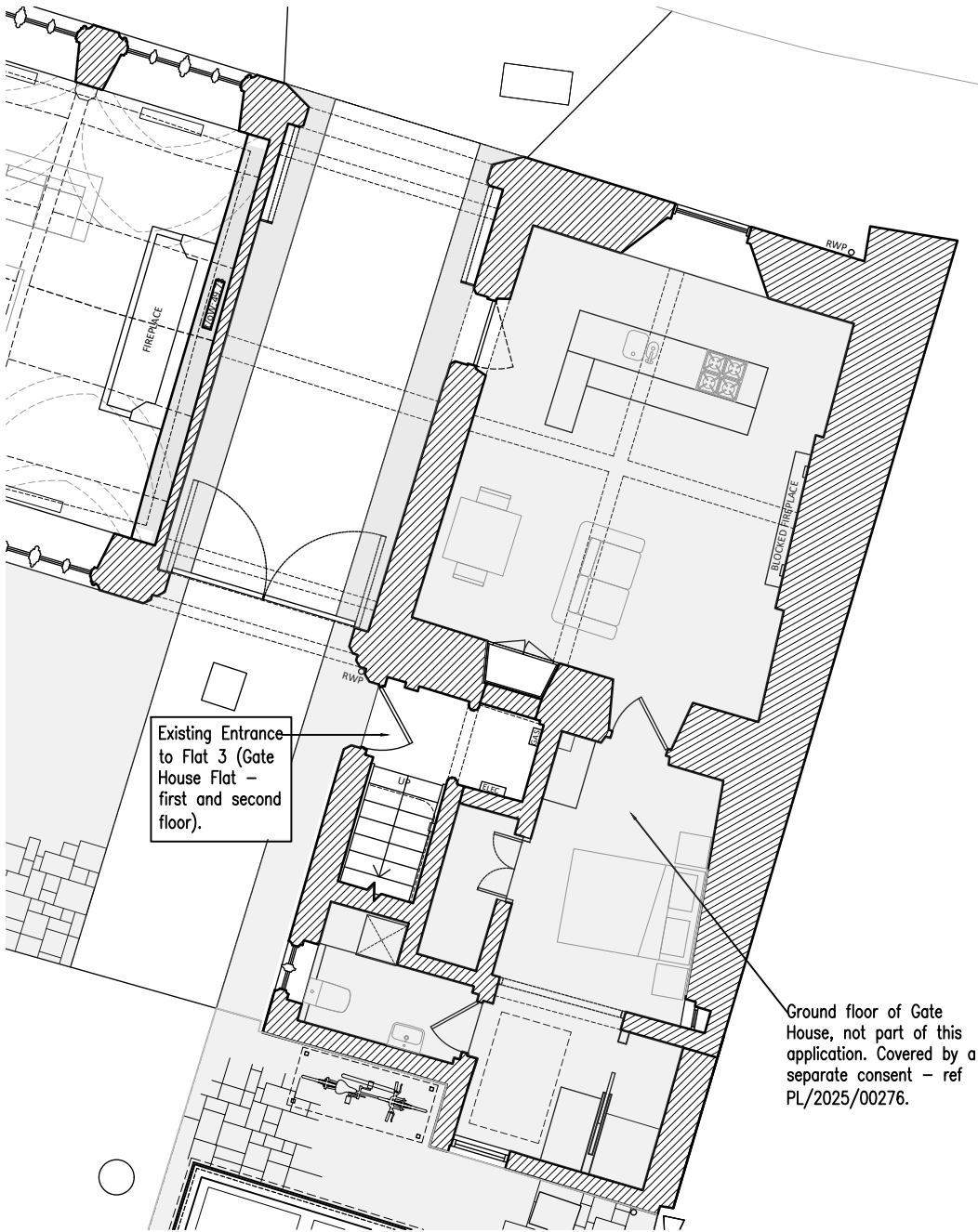
GATE HOUSE - GROUND FLOOR PLAN, SCALE 1:100@A2.
