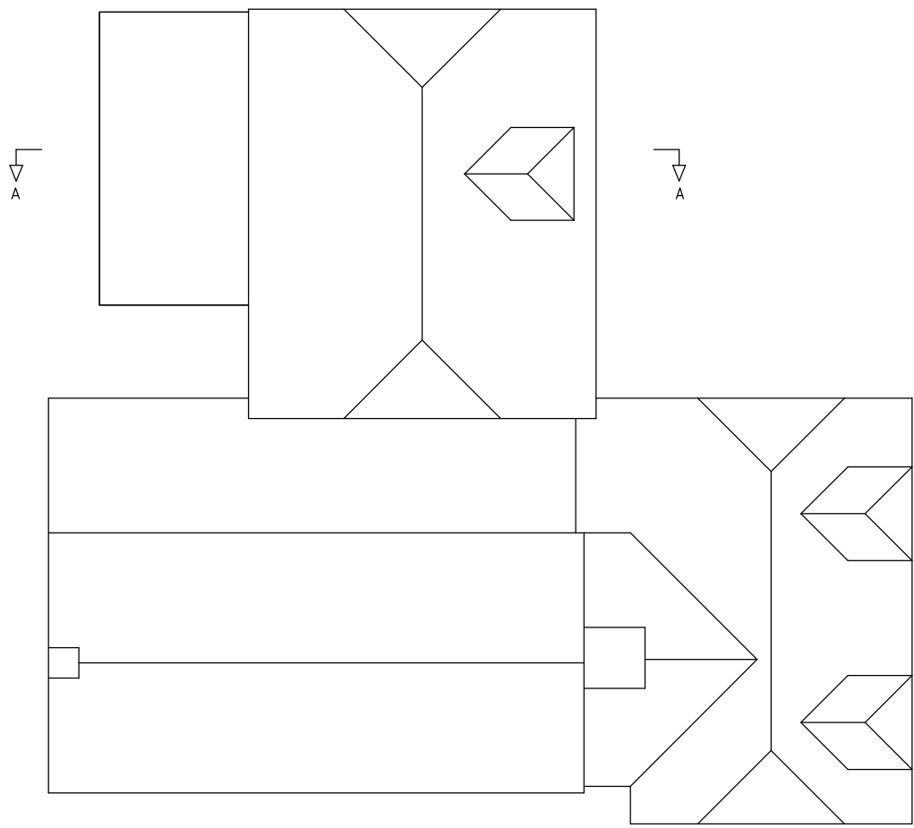
ROOF PLAN
