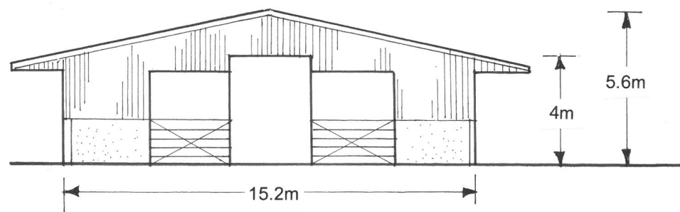
EAST & WEST ELEVATIONS
