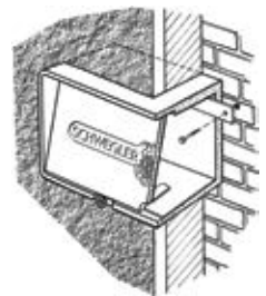
Flush-mounted ► in insulation with optional Fixing Bracket
