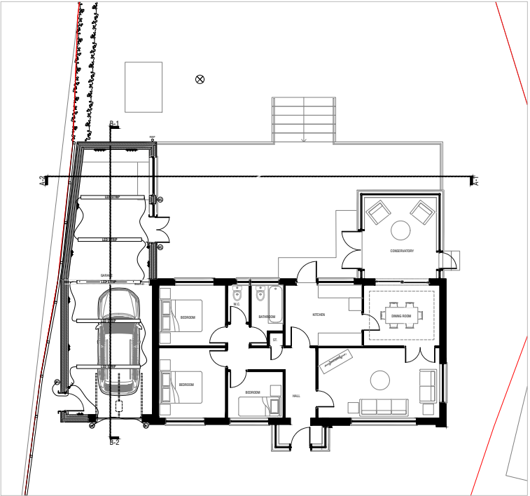
02 - Detailed Ground Floor Plan
