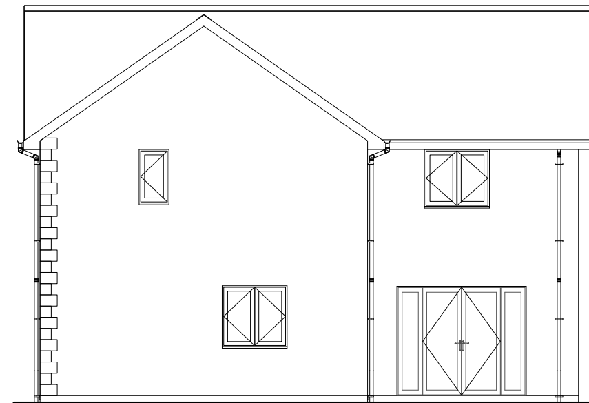
REAR ELEVATION
