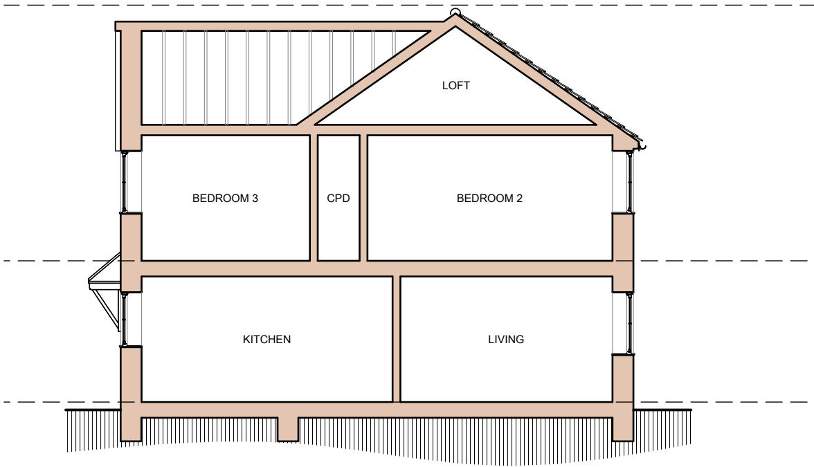
Side Elevation/Section BB - Plots 1&2 Proposed
