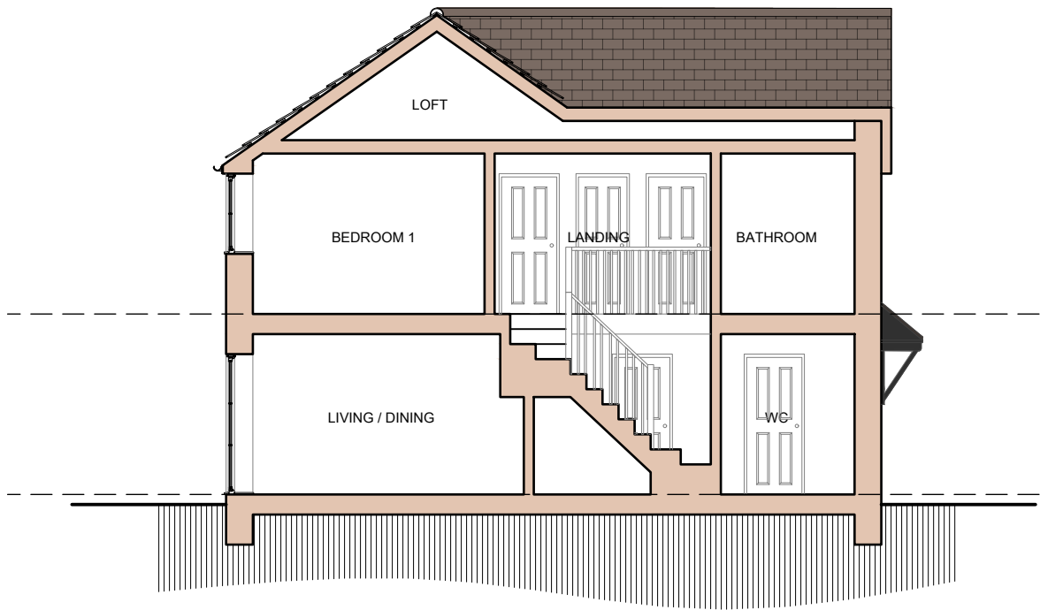
Section AA - Plots 1&2 Proposed
