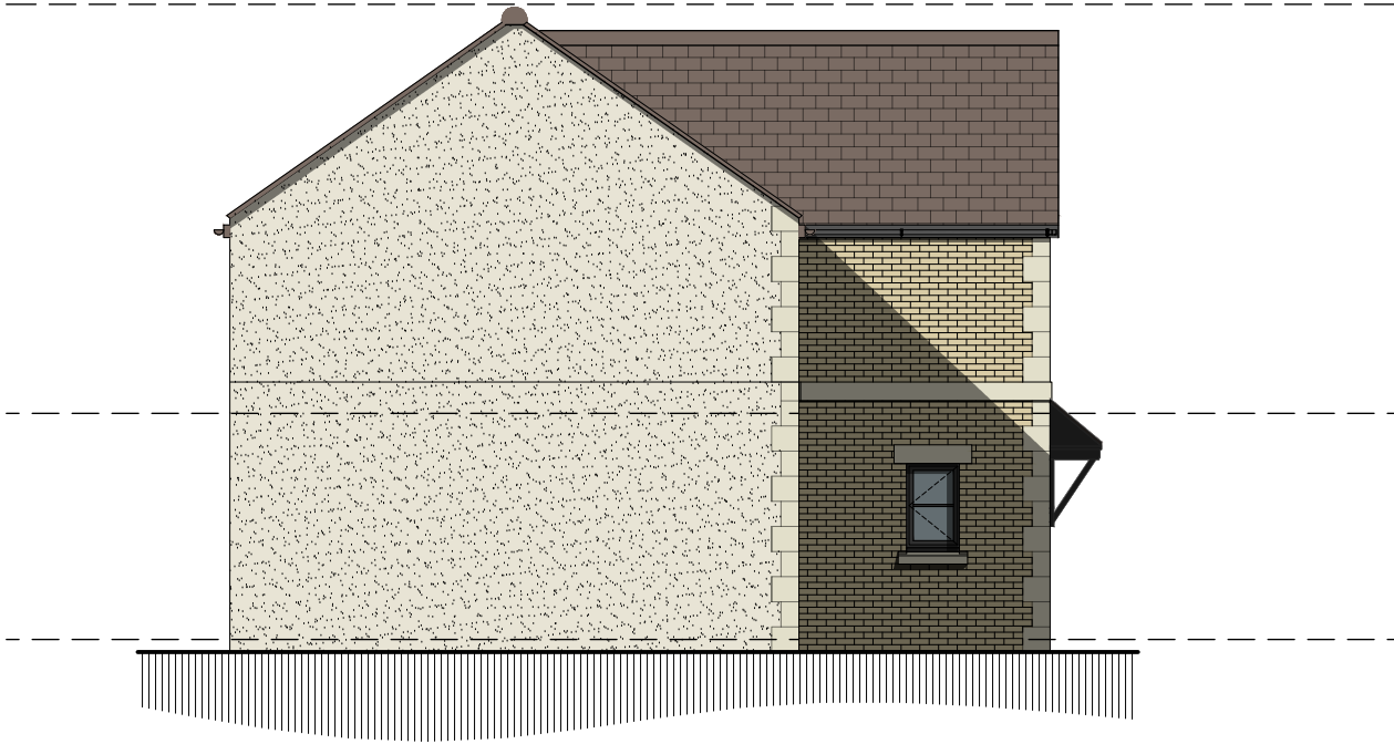
Side Elevation - Plots 1&2 Proposed
