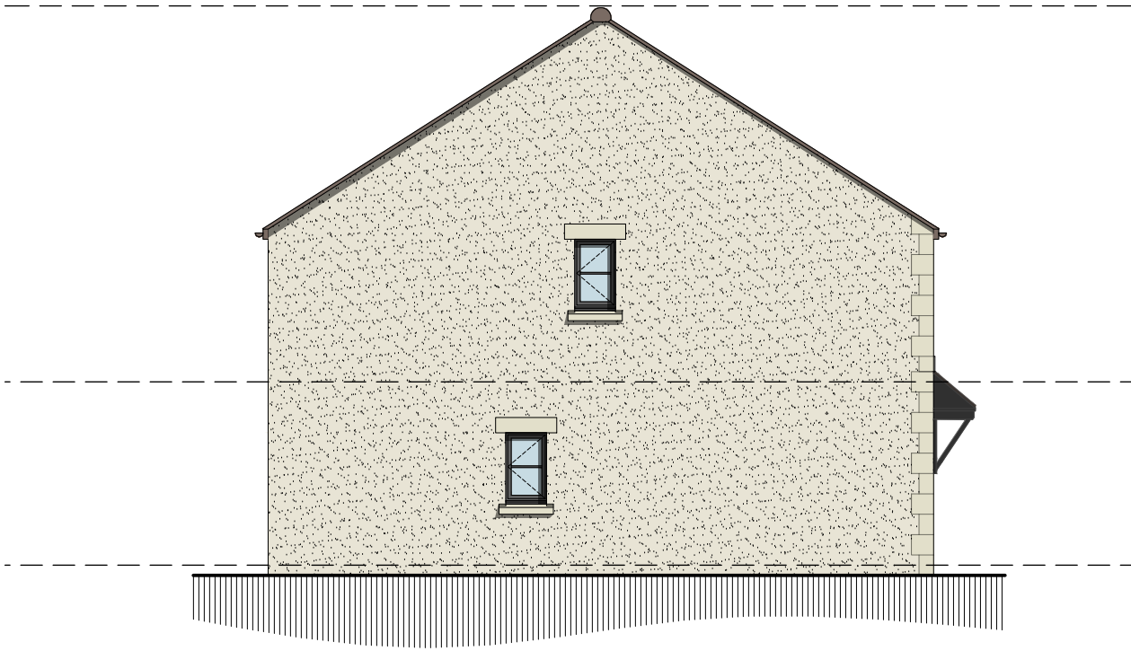
Side Elevation - Plot 6 Proposed
