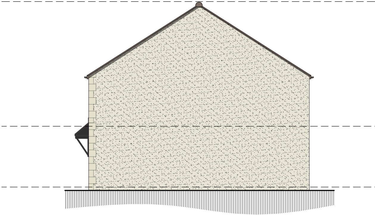
Side Elevation - Plot 5 Proposed
