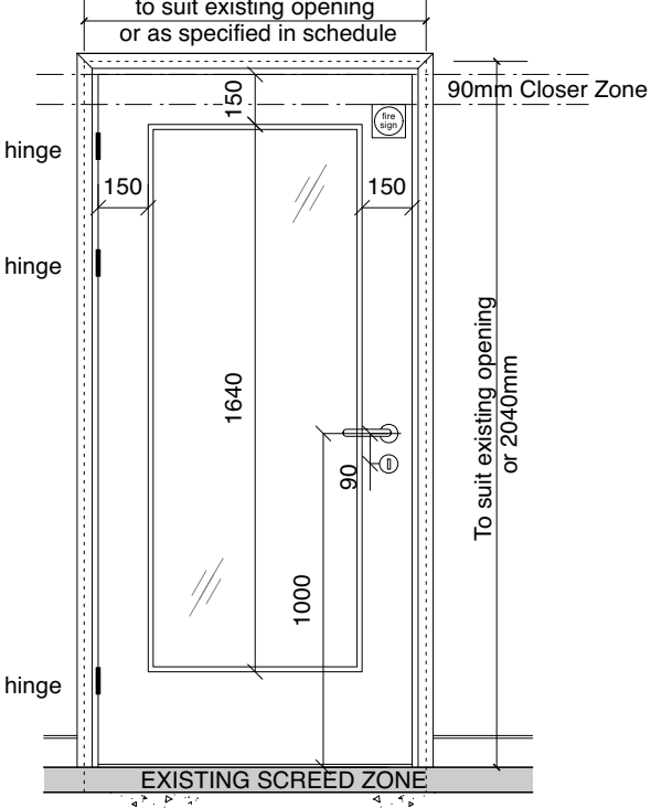
TYPICAL FULLY GLAZED DOOR (F)
