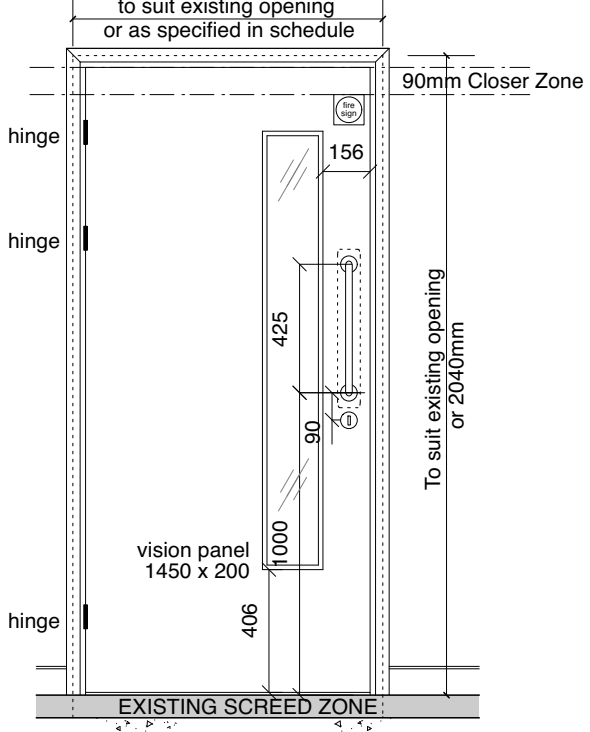
TYPICAL DOOR WITH SLIM VISION PANEL (VP-1)
