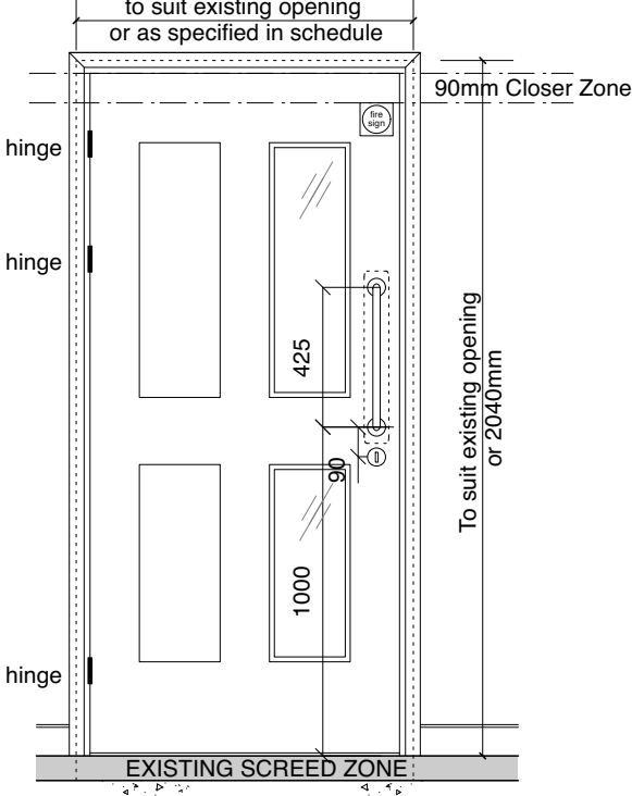
TYPICAL DOOR WITH VISION PANEL (VP-2)
