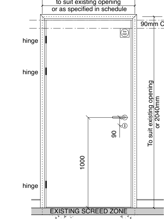
TYPICAL SOLID DOOR (S-1)
