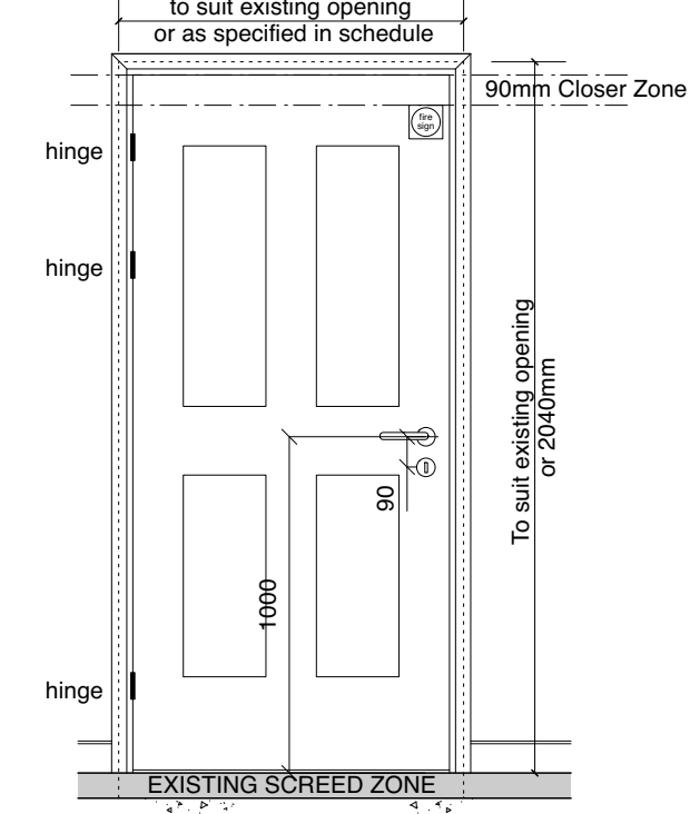
TYPICAL SOLID DOOR (S-2)
