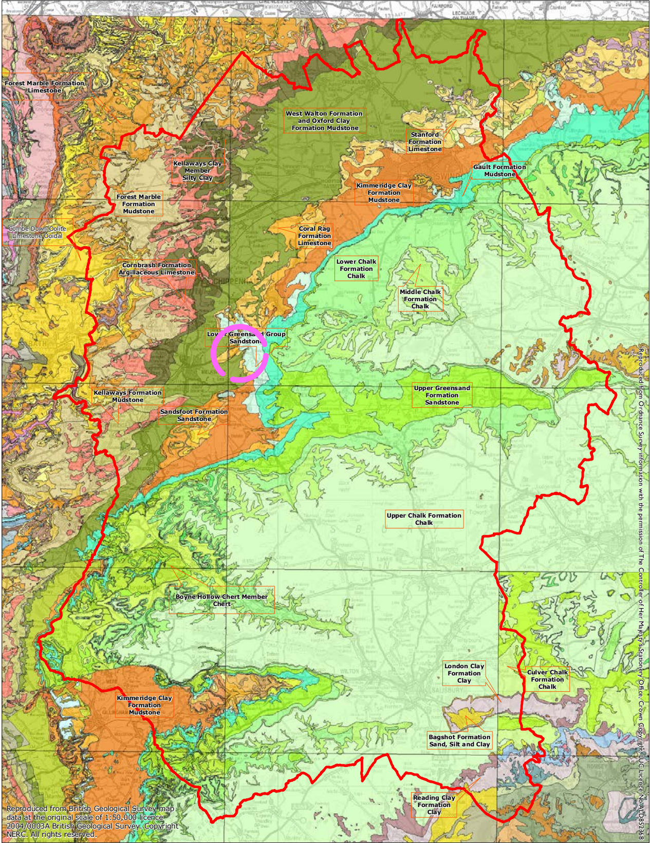
Figure 9: Solid Geology
