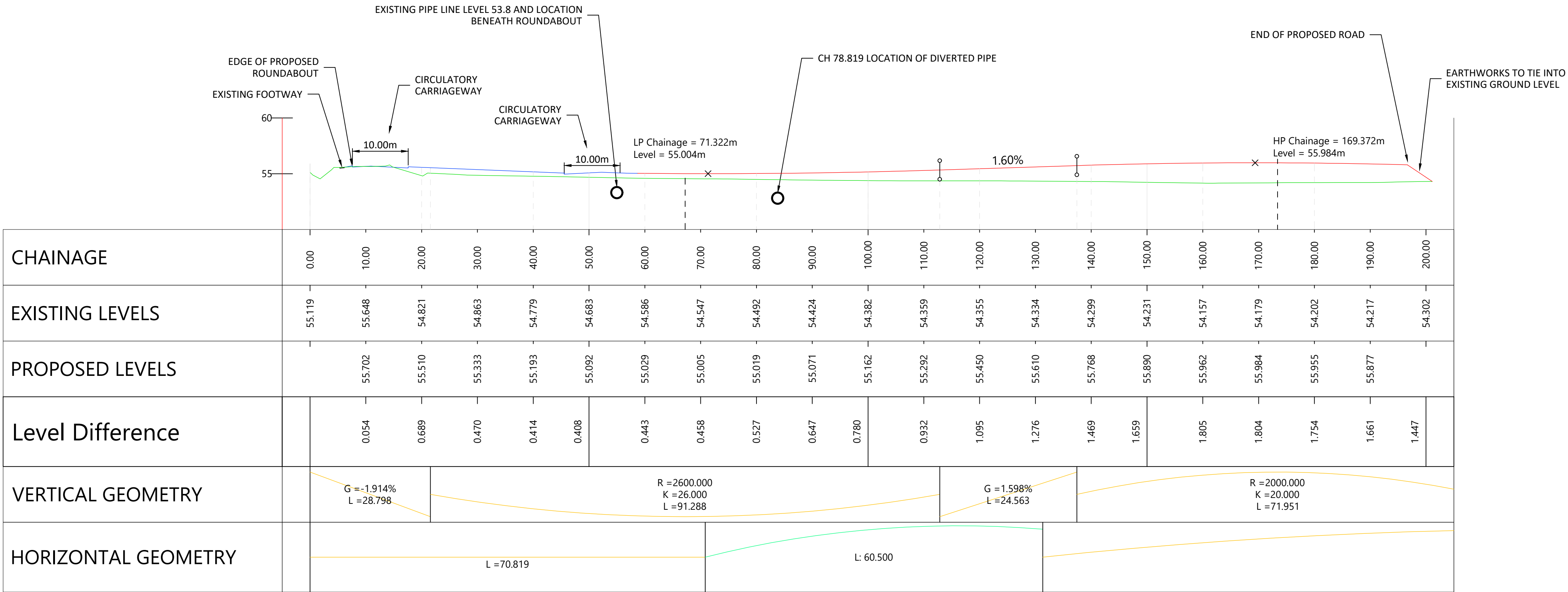
SPINE-ROAD-40MPH - LONGSECTION SCALE: H 1:500,V 1:250. DATUM: 50.000
