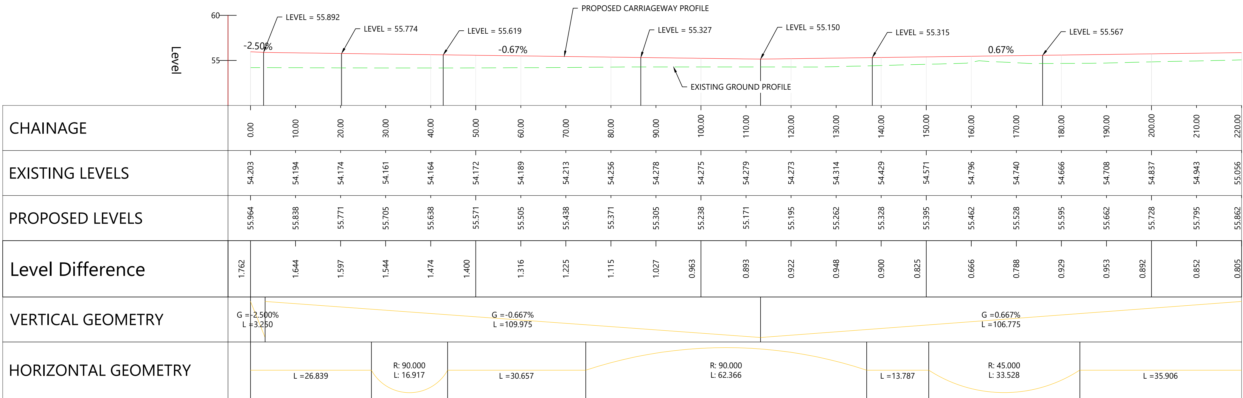
MINOR ARM VERTICAL ALIGNMENT - LONGSECTION SCALE: H 1:1000,V 1:500. DATUM: 50.000
