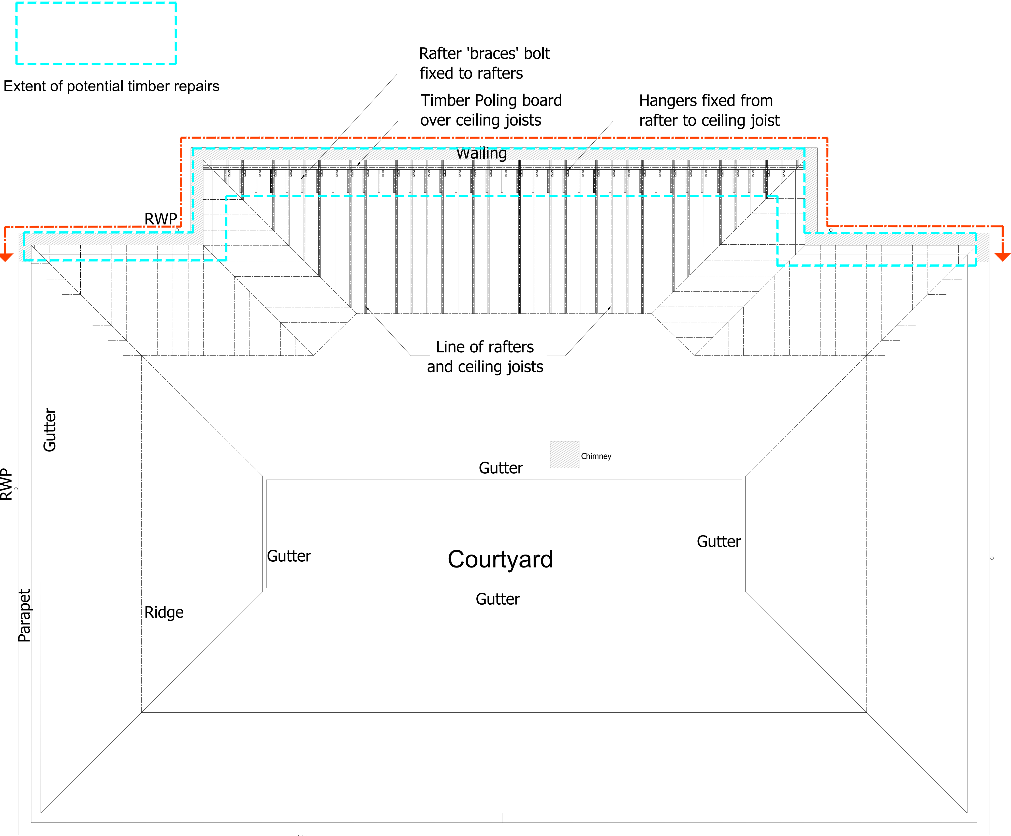
Roof Chord Layout (Scale 1:50)
