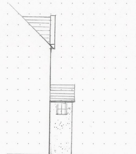
III. NORTH ELEVATION - EXISTING (CROSS SECTION OF SEMI-DETACHED)
